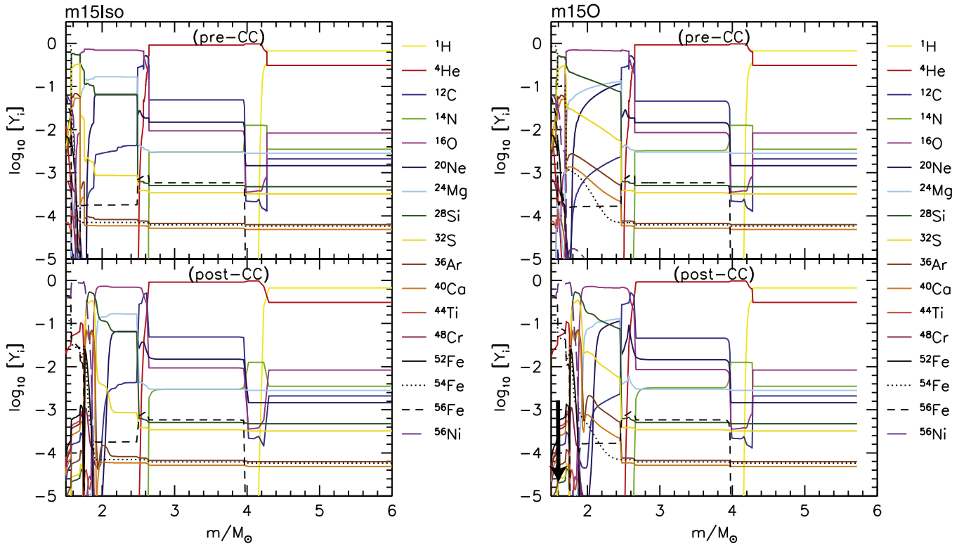
Figure 4. Left: composition profile for the 15 M_{\odot} model with steady mass loss (m15Iso). The top panel shows the composition of the inner 6 M_{\odot} prior to core collapse, while the bottom panel shows the composition for the same elements after core collapse. There is no mixing assumed in these models. Right: same as in the left panels, but for the model that underwent extreme mass loss during core oxygen burning (m15O). After evolving the models in the bottom panels for 400 yr with our ChN code, \sim 1 M_{\odot} of ejecta are shocked in the isotropic wind model, while nearly all the ejecta in the highly stripped model are shocked, as indicated by the arrow in the bottom right panel.
