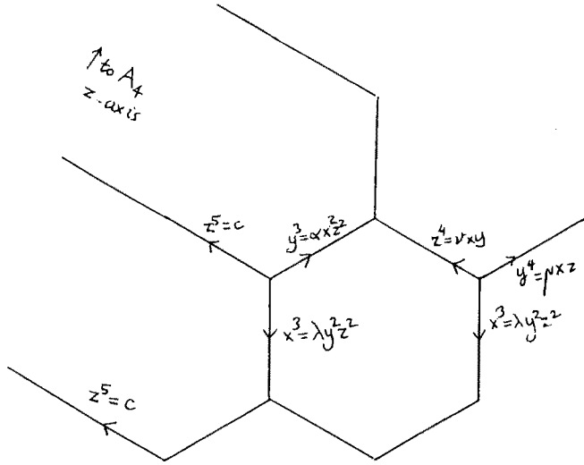
Figure 4: Two affine pieces near the hexagon at (3,1,1)
