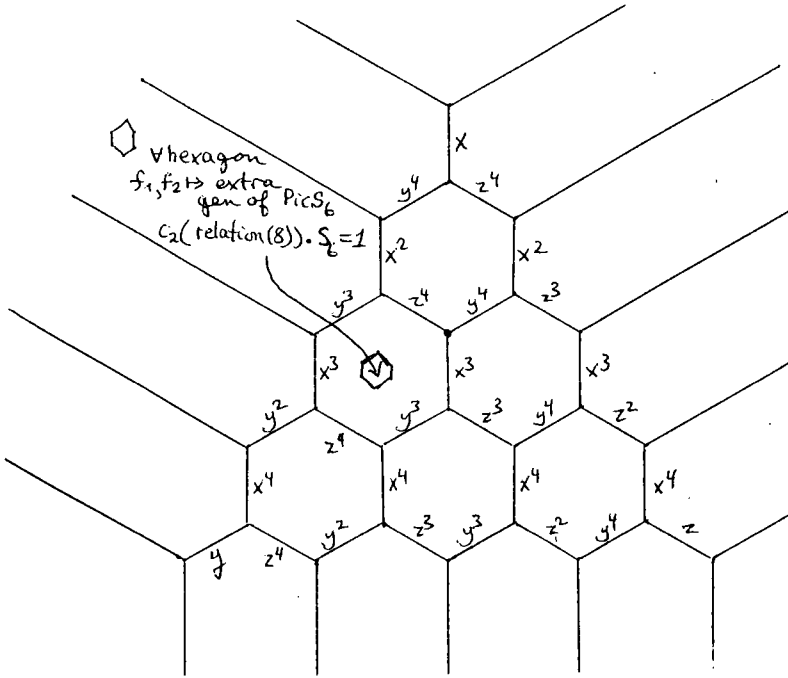
Figure 5: McKay correspondence
