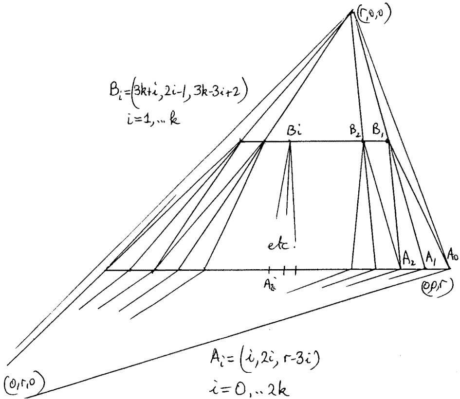
Figure 7: G\text{-Hilb} for \frac{1}{r}(1, 2, -3) . B_i is joined to A_{2i-2}, A_{2i-1}, A_{2i}
