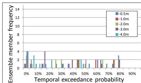
Fig.9 Ensemble member frequency according to temporal exceedance
