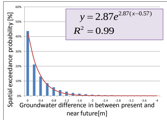
Fig.6 Spatial exceedance probability in average of all ensemble members and the approximate function
