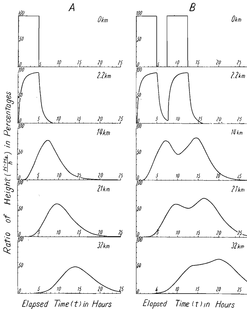
Fig. 1-A. Propagation of a solitary unit flood.
