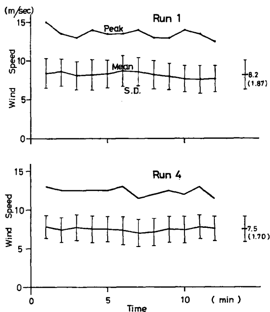
Fig. 4 Time variation of spacial mean wind speed.
