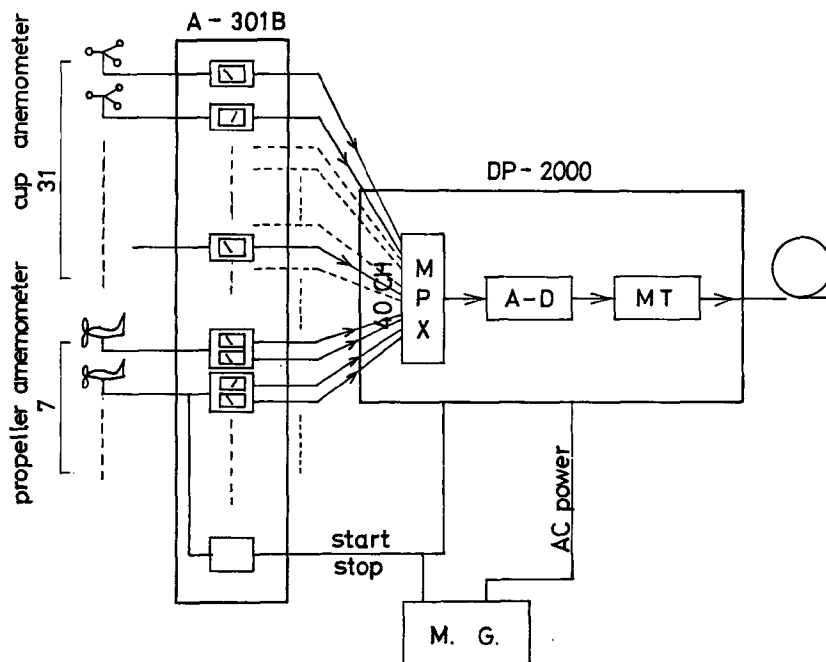
Fig. 3 Block-diagram of the observing system.
