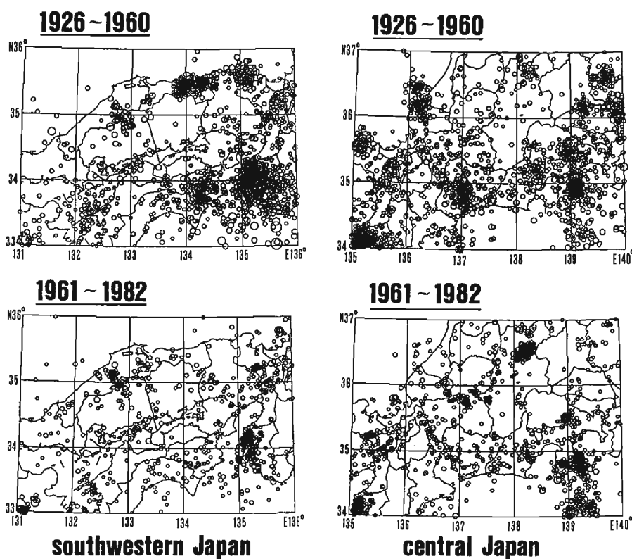
Fig. 13. The epicentral distributions for the two separated periods. Earthquakes of M \geq 3.0 and H \leq 30 km are plotted. Comparing these separated maps with the seismicity maps of Fig. 12, the seismic activity variation with time can be clearly recognized.
