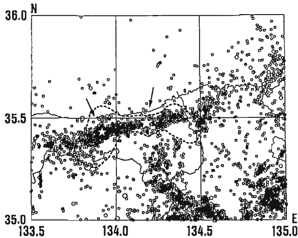
Fig. 7. Epicentral distribution in and around the Tottori plain from 1969 to 1987, obtained by the Tottori Microearthquake Observatory. The epicenter of the Tottori earthquake in 1943 is denoted by a big star with an arrow and that of the Central Tottori Pref. earthquake in 1983, by a small star with an arrow. The aftershock region of the Tottori earthquake defined by Hamada (1987) 8) is also shown by a dotted line.
