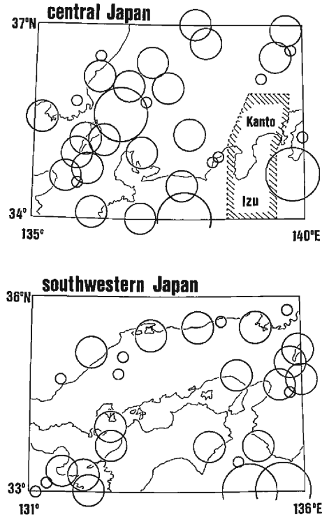
Fig. 11. Aftershock areas of the historical big earthquakes of M \geq 7 listed on Usami's table 18) and those of the recent big ones of M \geq 6.0 and H \leq 30 km listed in the J.M.A. catalogue. All these earthquakes were roughly classified into three groups depending on their magnitudes. The size of each circle corresponds to the aftershock surface area of an earthquake of M6.5 , M7.5 and M8.0 , respectively.
