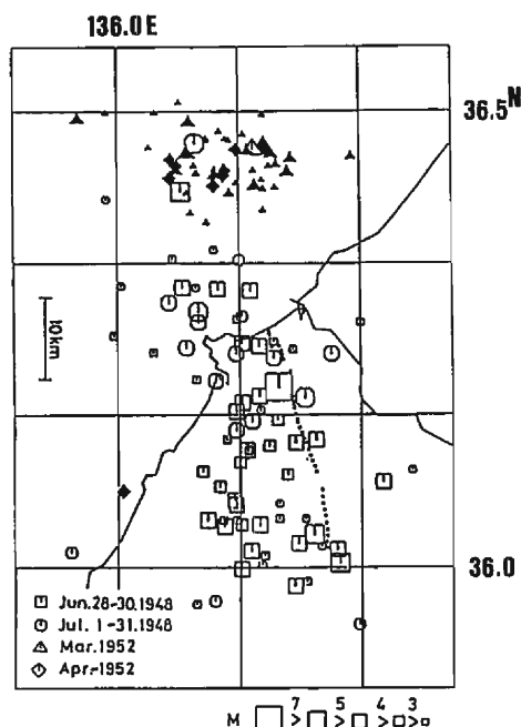
Fig. 2. Epicenters of the Fukui earthquake sequence (open symbols) and that of the Off Daishoji earthquake (solid ones). Both were relocated by Hamada (after Hamada (1987) 8) ).
