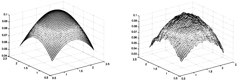
Figure 1: The analytical (left) and estimated (right) value functions at t = 0.09 around x = (\pi/2, \pi/2)^* .
