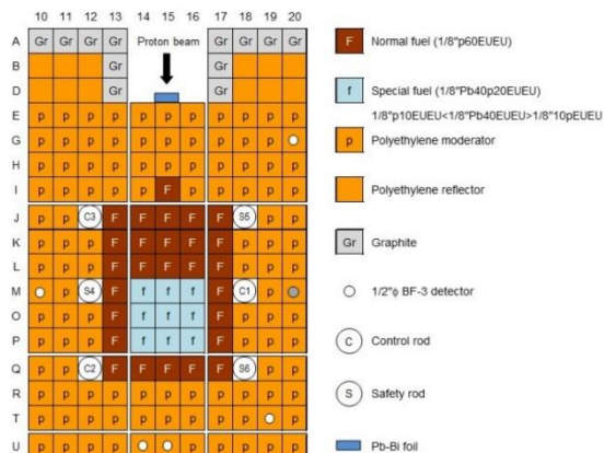
Fig. 1. Top view of the ^{235}\text{U} -fueled and Pb-zoned core
