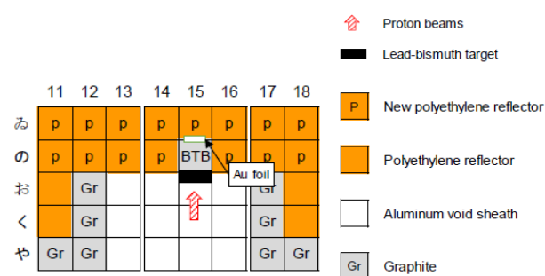
Figure 1. Loaded position of the BTB fission chamber and the Au foil in the A-core of the KUCA.
