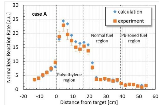
Fig. 2. Comparison of ^{115}\text{In}(n, \gamma)^{116\text{m}}\text{In} reaction rate distribution between measurement and calculation results at the subcriticality of 2487 pcm.
