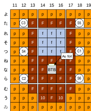
Fig. 1. Critical core for MA irradiation experiments.
