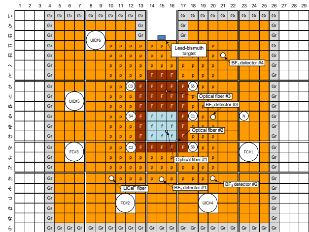
Fig. 1. Critical two-zoned core in KUCA (Case I).
