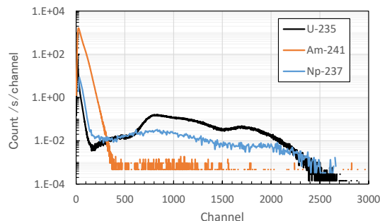
Fig. 2. Pulsed height from BTB fission chamber.
