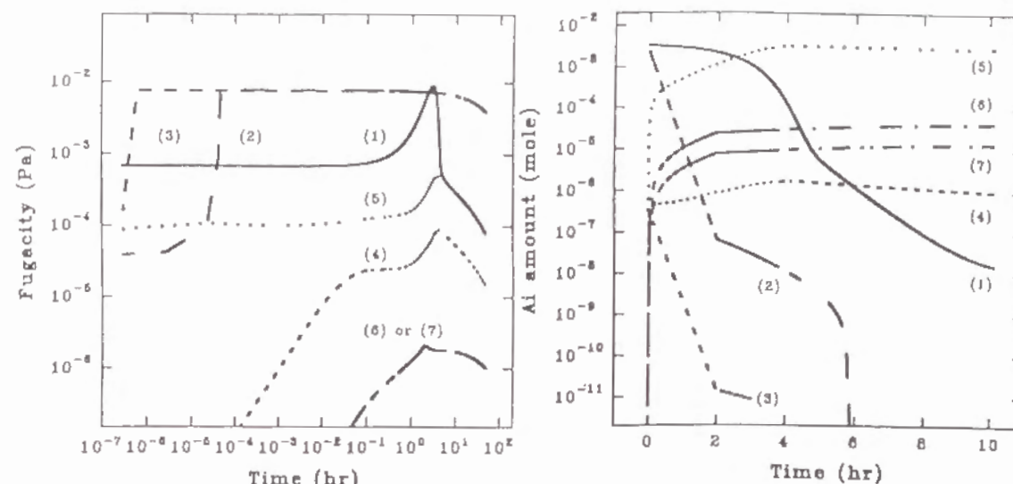
Figure 5-8. Fugacities of concerned compartment as a function of time. Water (1), droplets ( i = 2, 3 ), air (4), floor (5), wall (6) and ceiling (7).
