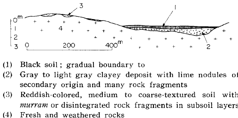
Fig. 2 Schematic cross section of a catenary soil distribution on non-calcareous basements
