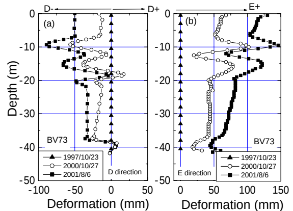
Fig. 10 Monitored results of borehole inclinometer at point BV73
