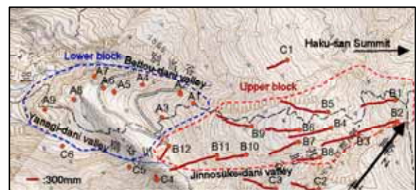
Fig. 8 Cumulative displacements of the landslide from 1994 to 2001
