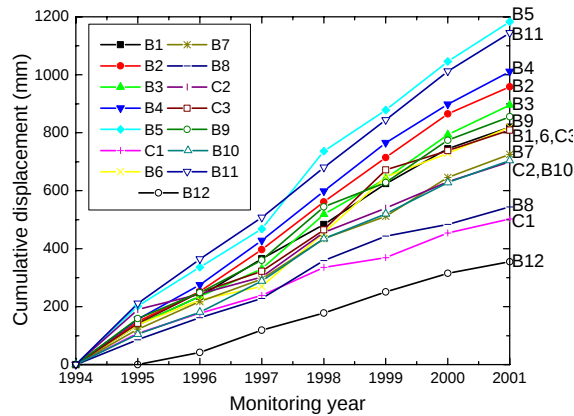
Fig. 9 Time series of cumulative displacements of survey points B1-B12 and C1-C3 from 1994 to 2001 (Measurement at point B12 started from 1995)
