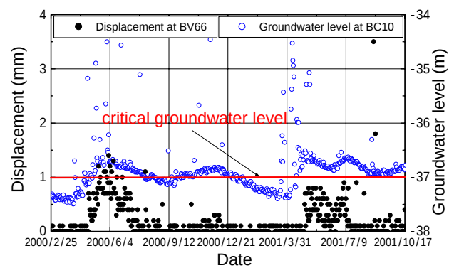
Fig. 14 Relationship between displacements measured at BV66 and groundwater level at BC10 indicating a critical groundwater level existing
