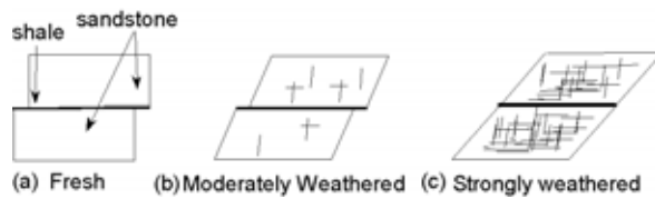
Fig. 12 Deformation model of the alternative layers of sandstone and shale at different weathering degrees
