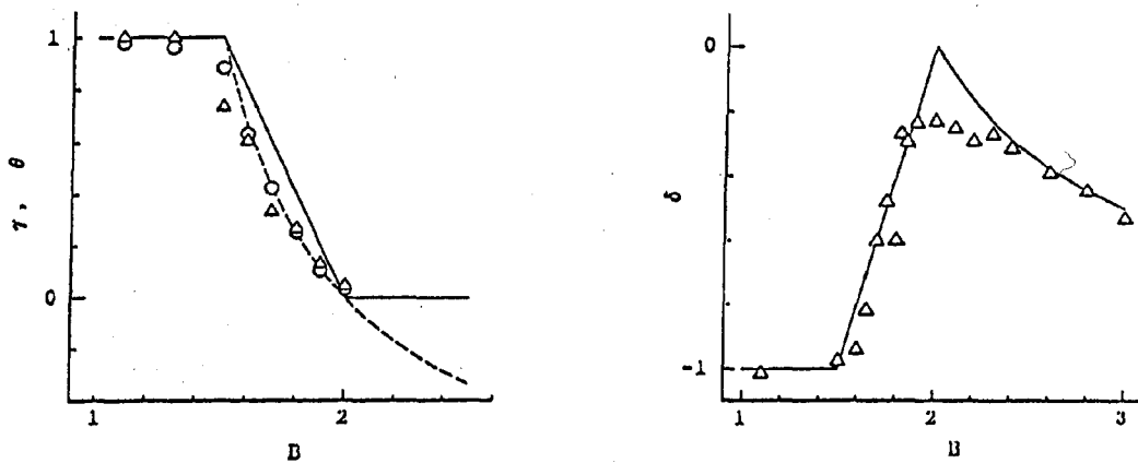
Fig.2 Scaling indices for the entropy function ( \Delta ), the Allan variance ( \square ) and the distribution of Lyapunov exponent ( \delta ).
