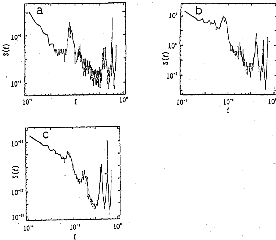
Fig.4 - PSD function of a lattice vibration model with small dissipation; the phase noise (a), the phonon number fluctuation (b) and the Rayleigh's function (c).
