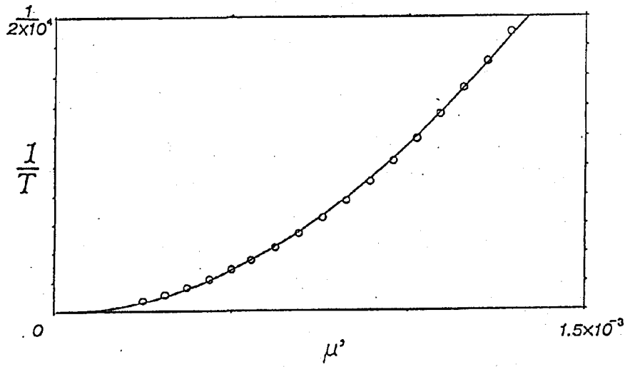
Fig.3 The Nekhoroshev bound for a lattice vibration model. \mu' stands for effective nonlinear parameter [8].
