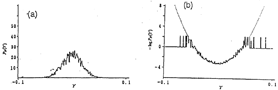
Fig.1 Large deviation properties ( B=1.1 ); (a) distribution function and (b) entropy function. The theoretical result is shown by a dotted line.
