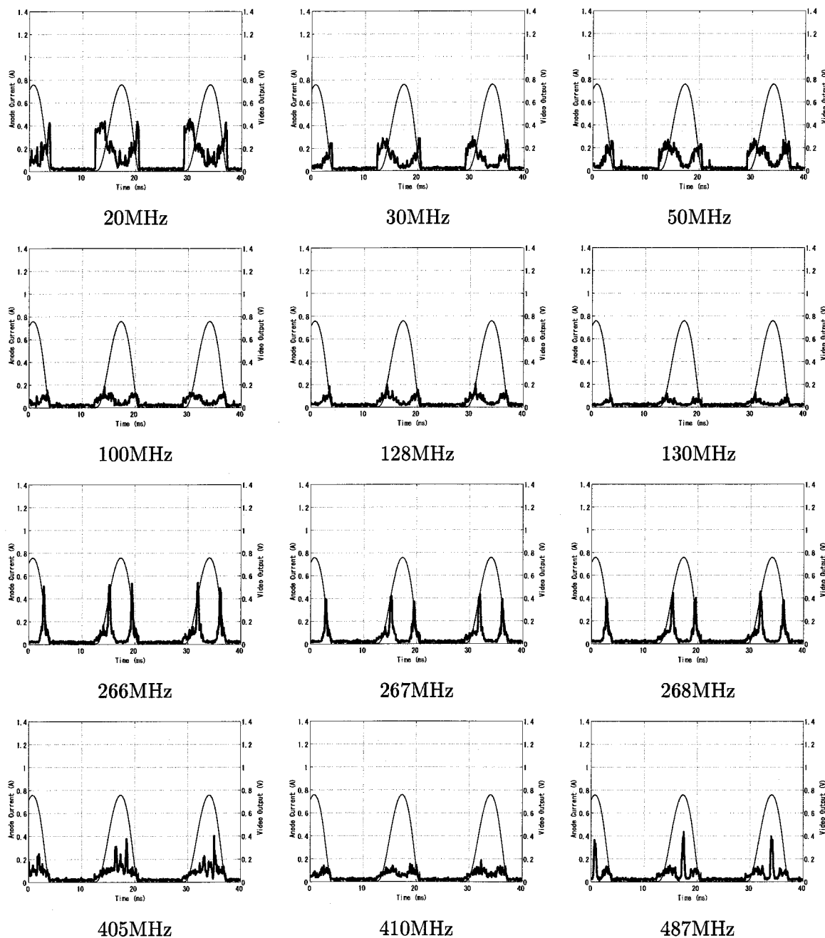
Figure A.10: Experimental results of the time domain analysis in the low frequency bands (2). Thick line and right axis: video output signal from the spectrum analyzer, thin line and left axis: the corrected anode current waveform of the reference magnetron.
