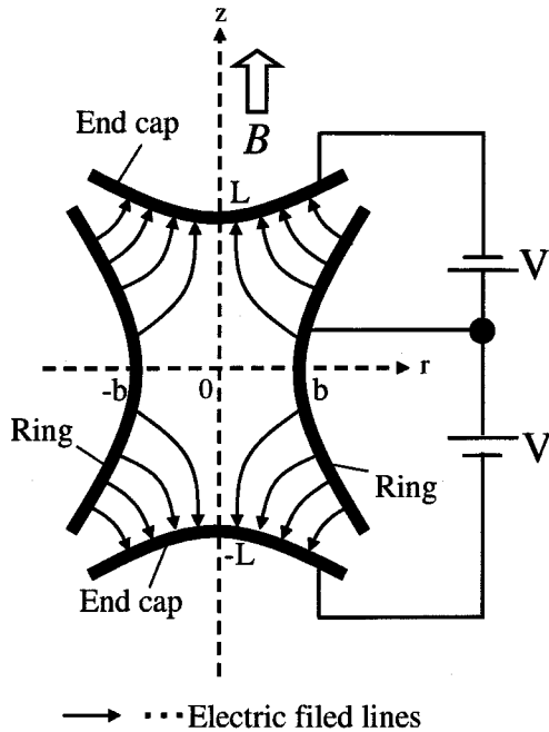
Figure 3.18: Cross-section view of a Penning trap in the r - z plane.
