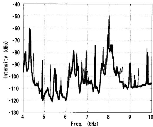
Figure 5.16: Relationship between the spurious noises and the anode current disturbance at I_f=10\text{A} . Thin line: I_b=250\text{mA} , and thick line: I_b=400\text{mA} , Resolution bandwidth: 100\text{kHz} .
