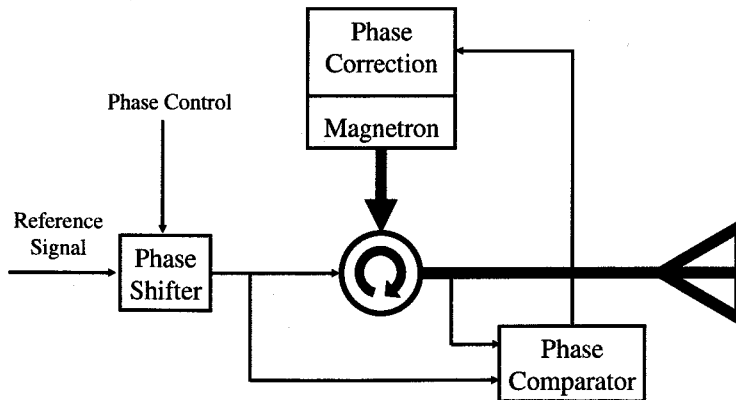
Figure 1.17: Basic configuration of a Phase-Controlled Magnetron (PCM) [38].
