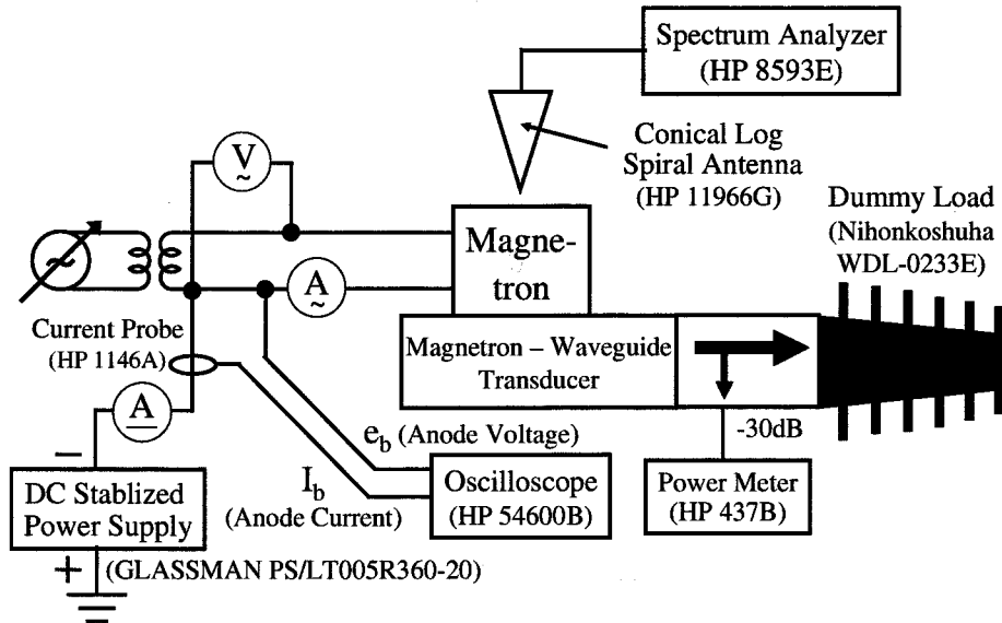
Figure 5.1: Schematic of a measurement system for obtaining the oscillation bandwidth of a magnetron.
