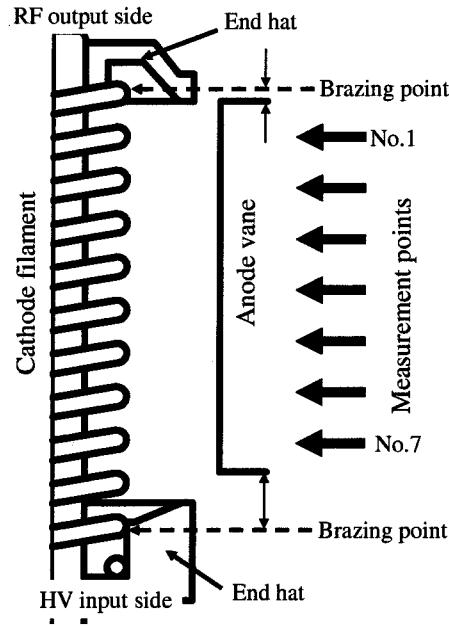
Figure 2.15: Brazing points between the cathode filament and the end hats.
