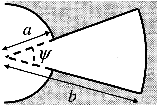
Figure 3.17: Annular-sector resonator.
