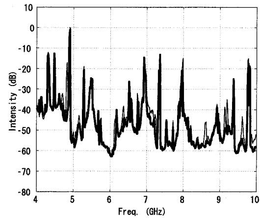
Figure 5.17: Relationship between the spurious noises and the influence of the AC magnetic field at I_b=250\text{mA} and I_f=10\text{A} . Thin line: AC power supply, and thick line: DC power supply, Resolution bandwidth: 100\text{kHz} .
