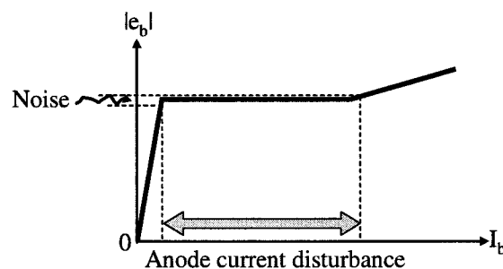
Figure 5.9: Anode current I_b disturbance by a small ripple noise on the anode voltage |e_b| .
