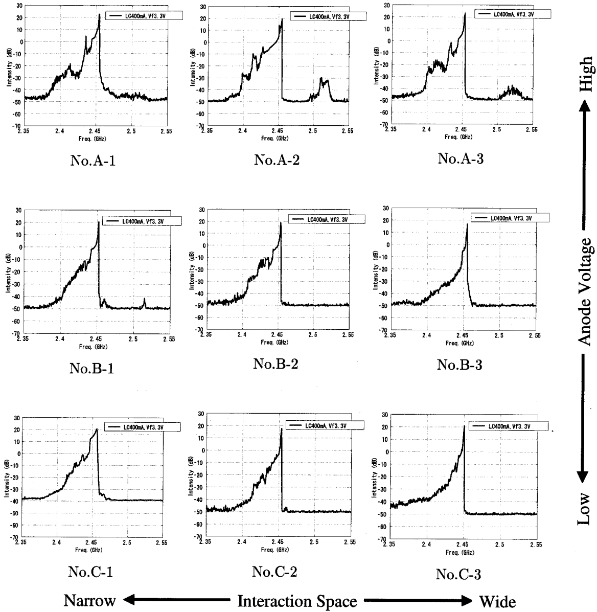
Figure 4.2: Measurement results of the magnetrons by the modifications of the interaction space and the anode voltage in the fundamental bands (2.35GHz–2.55GHz).
