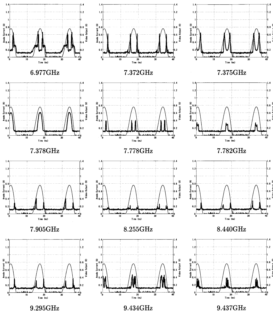
Figure A.6: Experimental results of the time domain analysis in the high frequency bands (3). Thick line and right axis: video output signal from the spectrum analyzer, thin line and left axis: the corrected anode current waveform of the reference magnetron.
