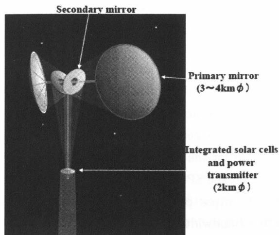
Figure 1.15: “Mirror-type” SPS concept – 2001 NASDA Reference System – [35].
