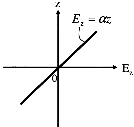
Figure 3.19: Axial electrostatic field at r = 0 in an ideal Penning trap. \alpha = 4V/(2L^2 + b^2) .
