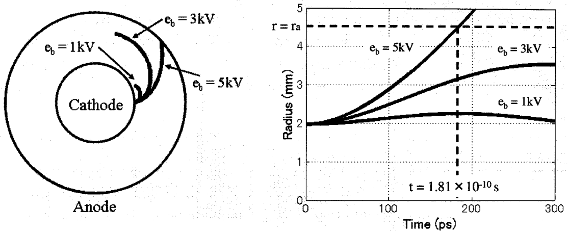
Figure 2.8: Trajectory of a single electron in a magnetron (left) and time variation of the radial position of the electron (right). The reference magnetron model 2M210M1F1 is used for parameters to solve the trajectory.
