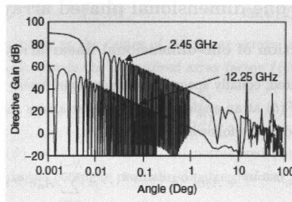
Figure B.1: Interference budget ( D/U ) calculation between a SPS ( U ) and a FSS satellite ( D ) for 12.25GHz [77].
