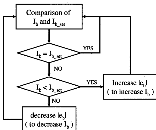
Figure 5.8: Flowchart of a prospective current controlling system of a DC stabilized power supply.
