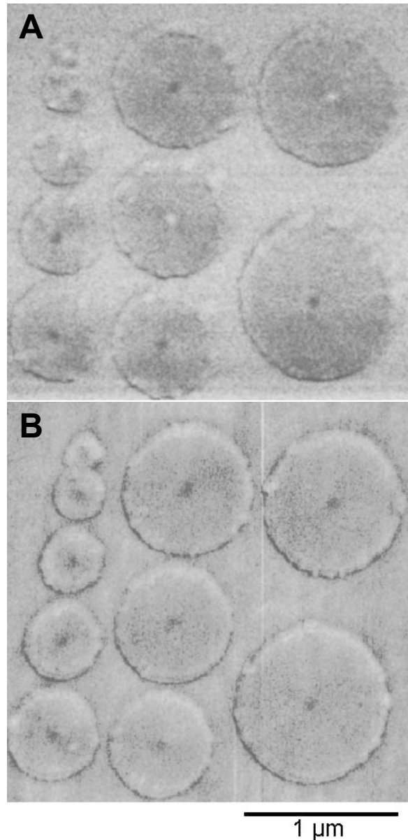
Figure 2. MFM image of an ensemble of 50-nm-thick permalloy dots with diameters varying from 0.1 to 1 \mu\text{m} after applying an external field of 1.5 T along an in-plane direction (A) and parallel to the normal (B).
