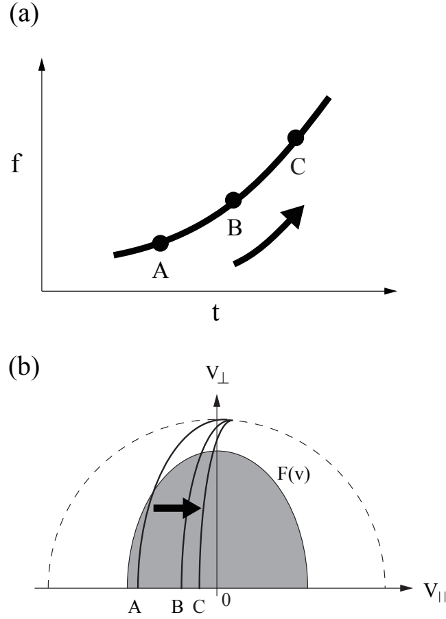
Figure 2. Schematic illustration of a frequency variation of a typical rising chorus element (a), and variation of resonance curve (b) superimposed on the velocity distribution function F(v) in the (v_{\parallel}, v_{\perp}) space, and the dashed semicircle is curve of speed of light. Resonance curves A, B, and C in panel (b) correspond to different frequencies A, B, and C in panel (a), respectively.
