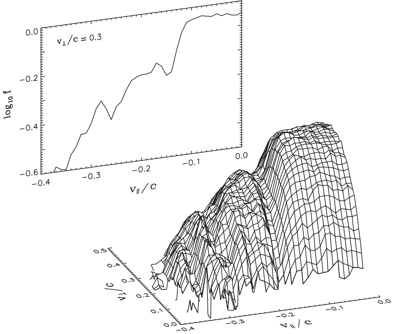
Figure 8. The distribution function f(v_{\parallel}, v_{\perp}) at time (iii) in Figure 4 and its cross section at v_{\perp} = 0.3c .
