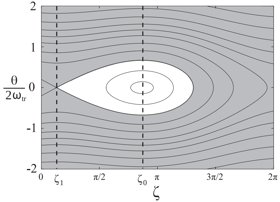
Figure 5. Trajectories of resonant electrons in the (\theta, \zeta) phase space for the inhomogeneity ratio S = -0.41 .
