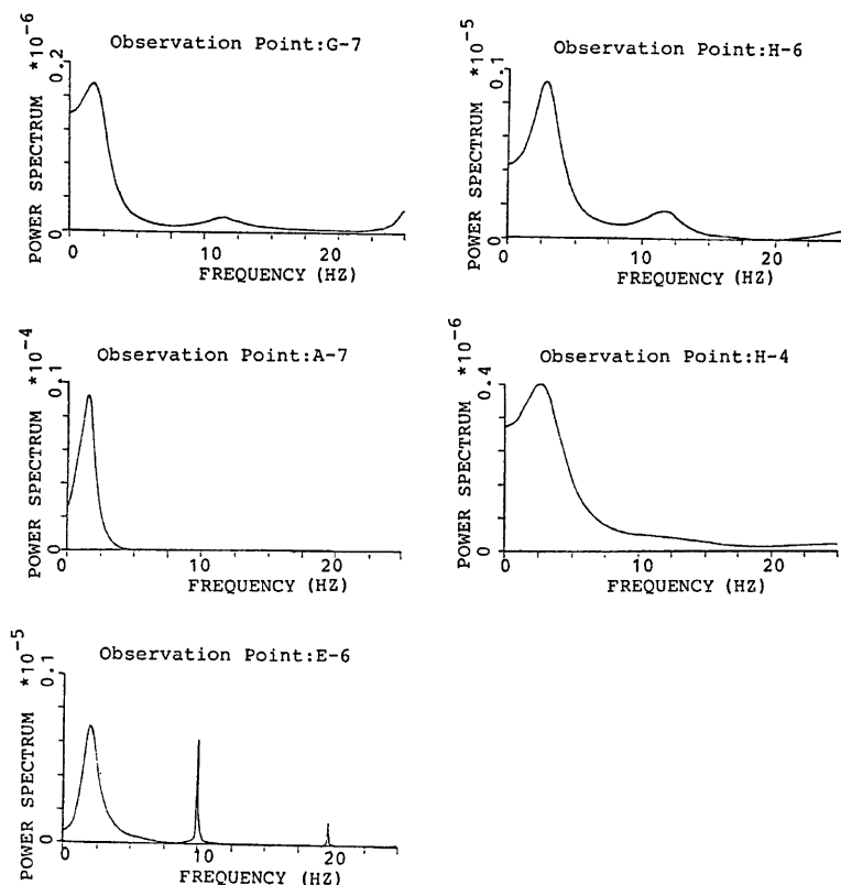
Fig. 8 Power spectra obtained from AR·MA (8, 8) process (on the ground).
