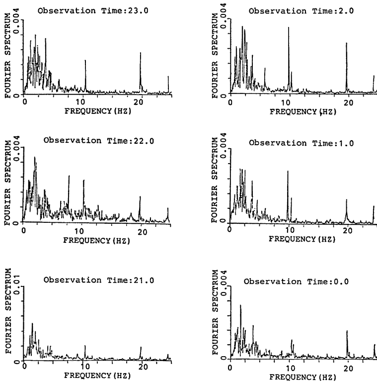
Fig. 4 Fourier spectra on the top of quaywall for different observation time (E-6 site).
