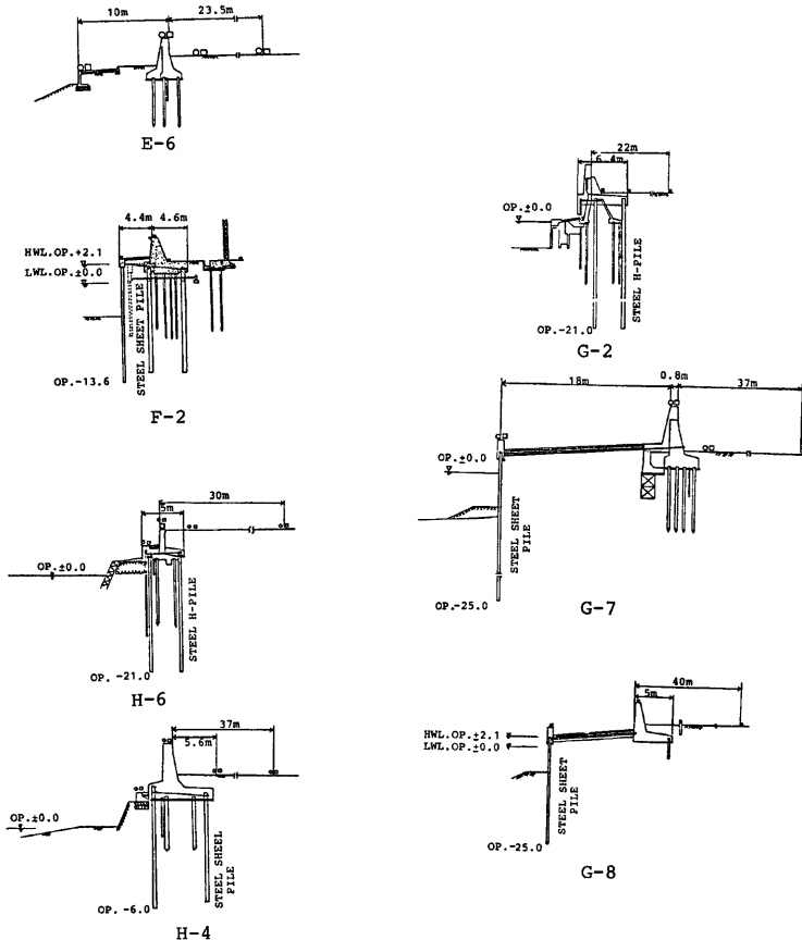
Fig. 3 Cross sections of observation sites.
