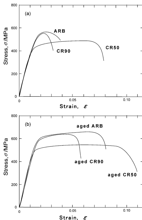
Fig. 4 Stress-strain curves of the Cu-Ni-P-Zr specimens, (a) CR50, CR90 and ARB, (b) CR50 aged at 400^\circ\text{C} for 1 h and CR90 and ARB at 350^\circ\text{C} for 30 min.
