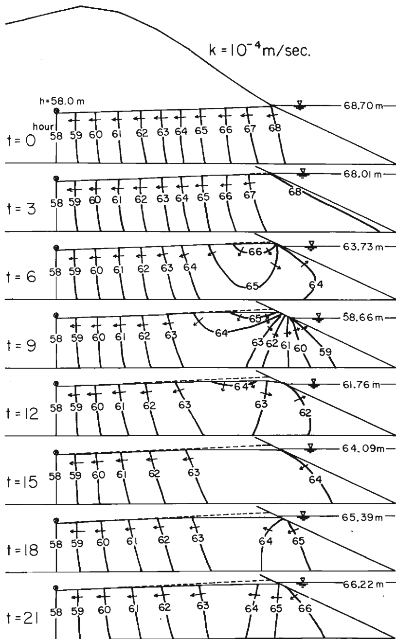
Fig. 13(A). Variations of equi-potential inesl of ground water for k=10^{-4} m/sec (arrow shows the stream direction).
