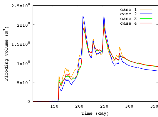
Fig. 6 Flooding volume time series.
