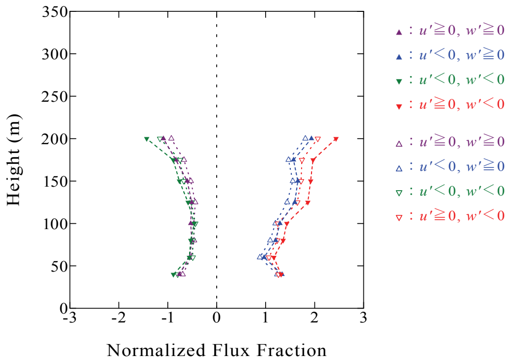
Fig. 5 Profiles of the flux fraction in each quadrant based on the Doppler sodar data for the observation case on Dec. 8, 1998 at Shionomisaki. Values are normalized with respect to the total u'w' at the lowest level. Averaging time is 54.6min (closed symbols) and 27.3min (open symbols)
