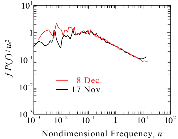
Fig. 4 Power spectrum on Dec. 8 and Nov. 17, 1998 at Shionomisaki
