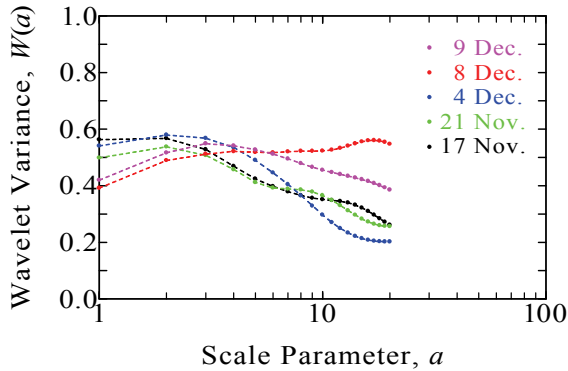
Fig. 3 Wavelet variance spectrum for each case in 1998 at Shionomisaki
