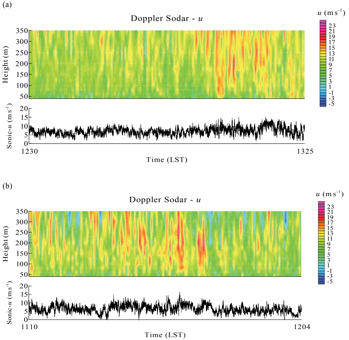
Fig. 1 Time-height cross section of the streamwise velocity component in the horizontal plane ( u ) observed by the Doppler sodar and the corresponding time series of the same component of velocity measured by the sonic anemometer-thermometer for part 1 of the observation case. (a) on Nov. 17 and (b) on Dec. 8, 1998 at Shionomisaki
