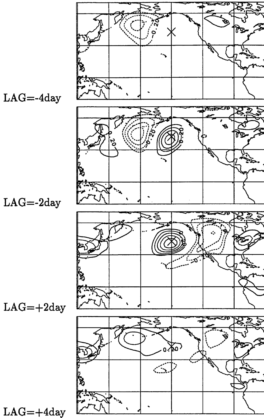
Fig. 3. Lag-correlation between the 20 - 30 day variations of the 300 hPa streamfunction at the base point (42.5°N, 150°W) and the 20 - 30 day variations of the 700 hPa streamfunction. Contour intervals are 0.1, and negative values are dashed. Correlations between - 0.1 and 0.1 are not contoured.
