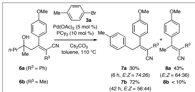
Equation 2
