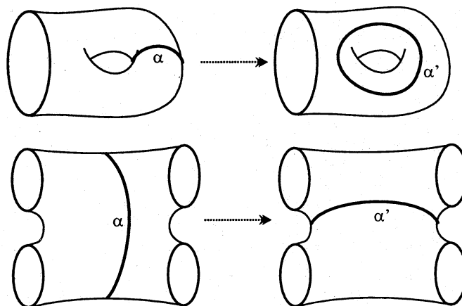
FIGURE 2. The two types of elementary moves.
