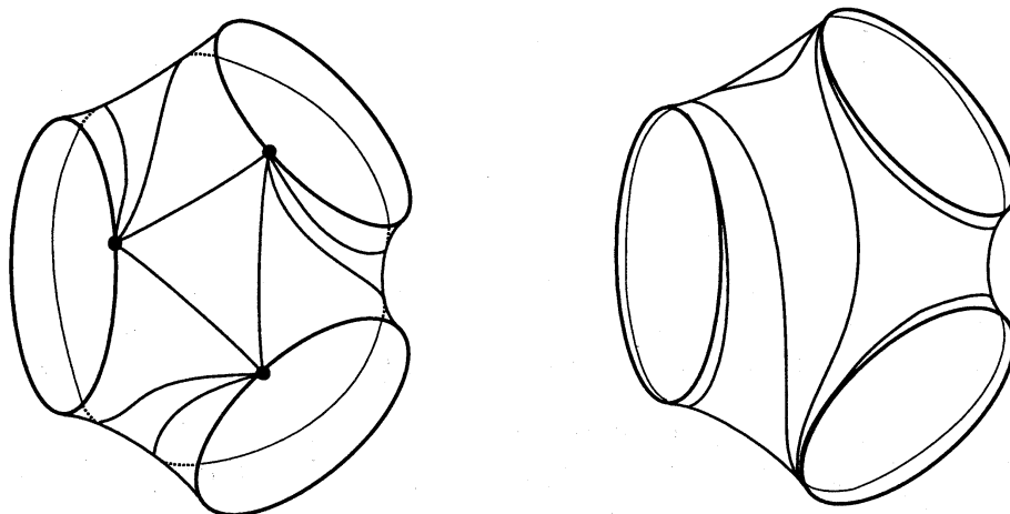
FIGURE 1. The lamination obtained by spinning a triangulation around a curve system. The picture shows one pair of pants in a decomposition.
