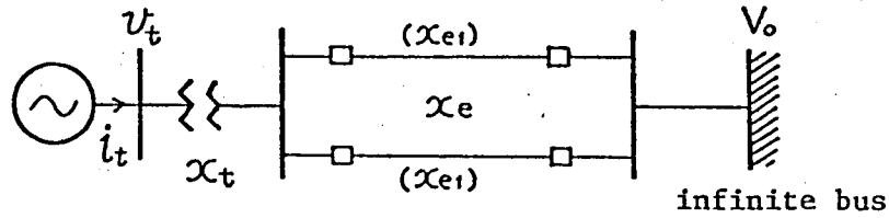
Fig.7-3-1 Model of one machine system
