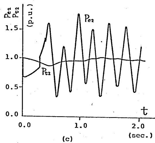
Fig.3-4-4 Transient unstable case of model system
