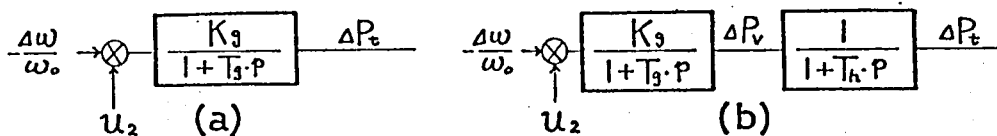
Fig.2-4-2 Simplified model of governor
