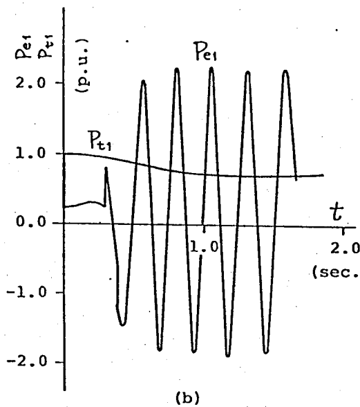
Fig.3-4-4 Transient unstable case of model system
