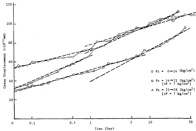
Fig. 6. Creep Displacement of Loading Plate.
