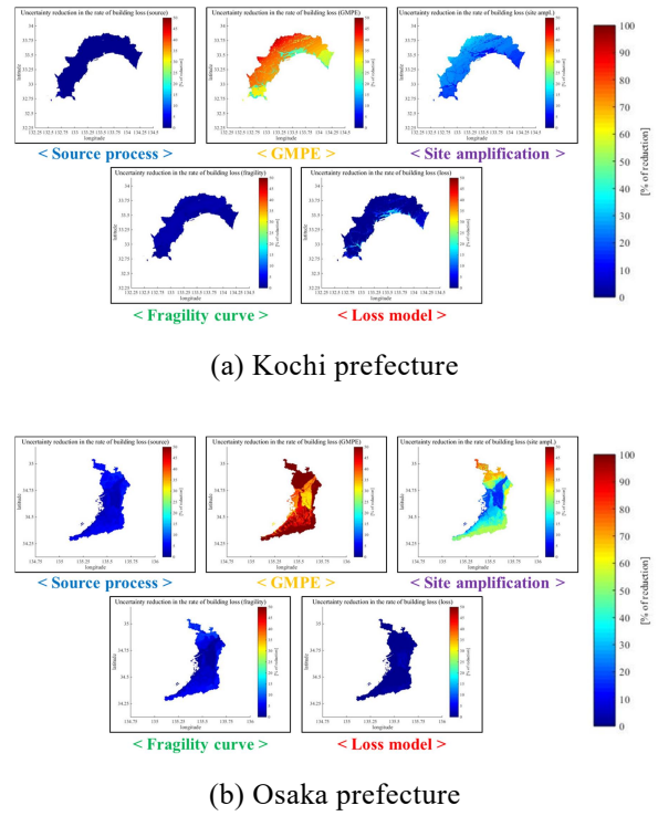
Fig. 23 Results of sensitivity analysis - Uncertainty reduction rate of building losses
