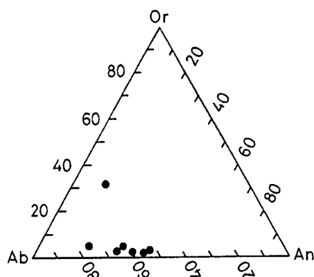
Fig. 8a. Or(KAlSi 3 O 8 )-An(CaAl 2 Si 2 O 8 )-Ab(NaAlSi 3 O 8 ) diagram for feldspars in I 0 sample.
