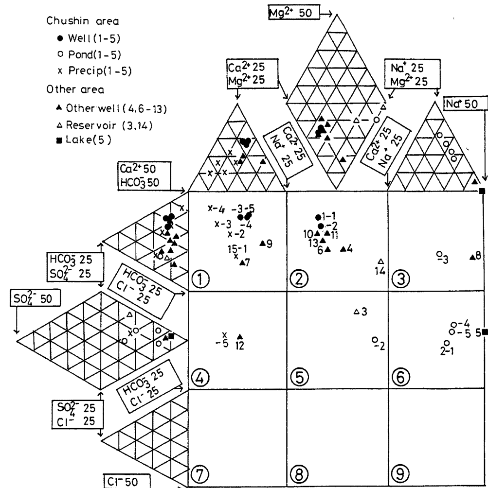
Fig. 3. Water types grouped using a expanded Durov diagram for natural waters: ①, fresh recharge water; ②・③, ion exchanged water; ④・⑤, simple dissolution or mixing; ⑥, brachish water.
