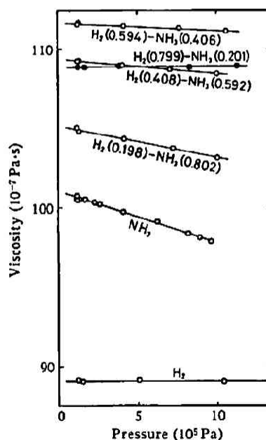
Fig. 2 Viscosity of hydrogen-ammonia system at 25°C
