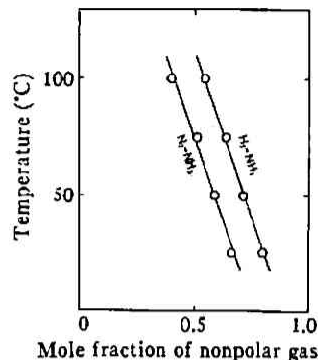
Fig. 8 Relation between temperature and x_H
