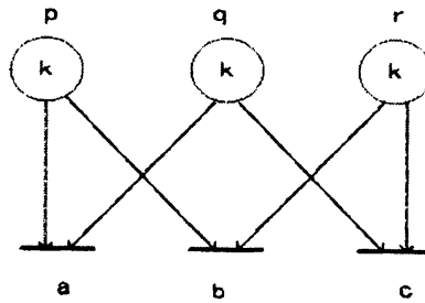
Fig. 3: A Petri net generating L_{\Omega,k} .
