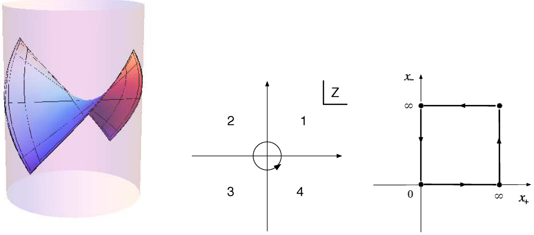
Figure 2. 4-cusp minimal surface in AdS_3 (left), world-sheet z -plane (middle), and surface boundary in the (x^+, x^-) -plane (right).
