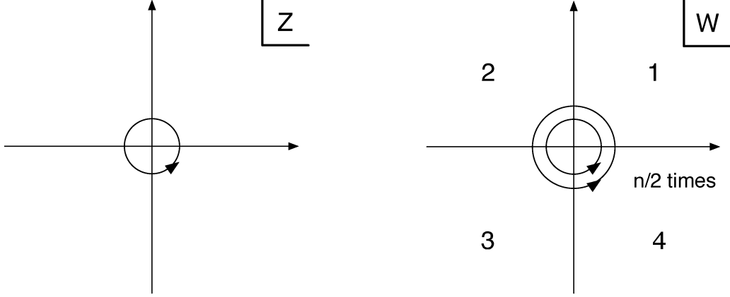
Figure 3. Rotation far from the origin in the z - and w -planes.
