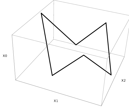
Figure 1. Boundary of a minimal surface on the AdS boundary. The axes in the figure represent the Poincaré coordinates (x^1, x^2, x^0) .
