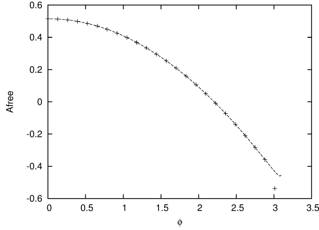
Figure 4. Plot of A_{\text{free}} := -F as a function of \phi for |Z| = 0.1 and \varphi = -\pi/48 from numerical results (+) and the high-temperature expansion (5.3) (dashed line).
