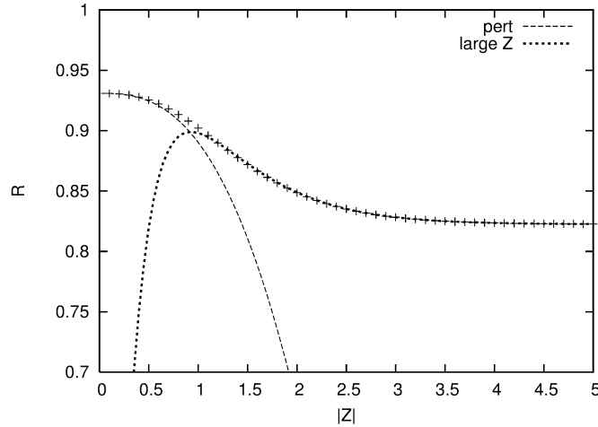
Figure 5. Plot of the remainder function \mathcal{R} as a function of |Z| for \phi = 0 and \varphi = -\pi/48 from the UV expansion (5.5) (dashed line), the first order IR expansion (dotted line) and numerical results (+).
