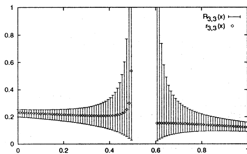
Fig.1 r_{3,3}(x) , R_{3,3}(x)
