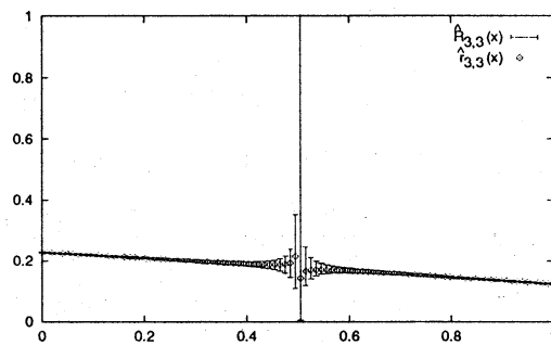
Fig.2 \hat{r}_{3,3}(x) , \hat{R}_{3,3}(x)
