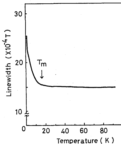
Fig. 9. Linewidth of the low temperature EPR of the TEMPAD biradical. T_m indicates the temperature where the susceptibility exhibits maximum.
