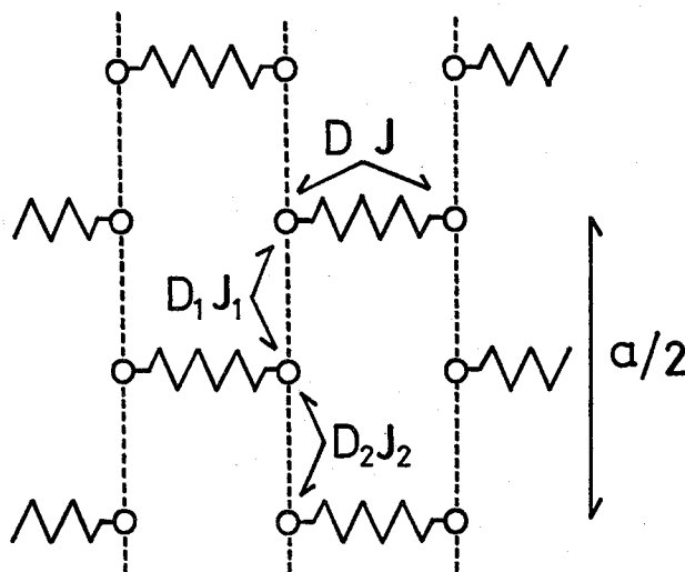
Fig. 2. Magnetic interactions in TEMPAD biradical. D and J mean intra-molecular dipolar and exchange interactions respectively. D_1 , J_1 , D_2 , and J_2 mean inter-molecular interactions. \bigcirc in the figure represents N-O nitroxyl group in a molecule.
