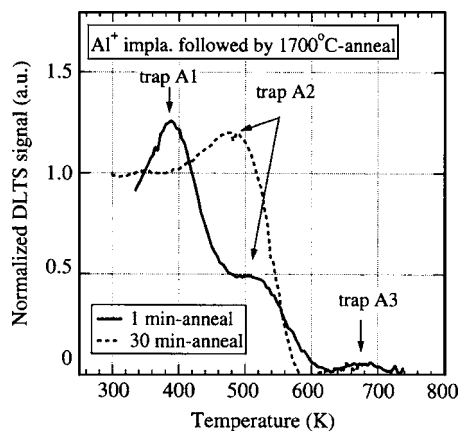
FIG. 2. DLTS signals from the samples implanted with \text{Al}^+ and annealed at 1700^\circ\text{C} .
