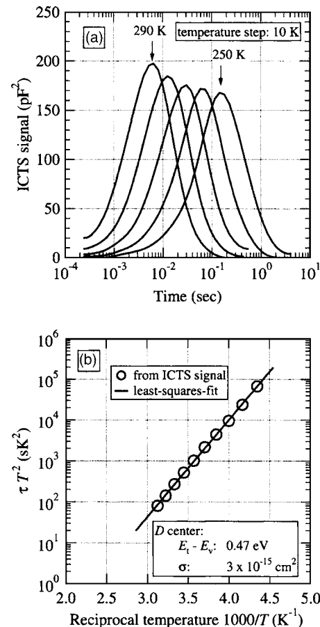
FIG. 4. ICTS data of the samples implanted with B + and annealed at 1700 °C: (a) ICTS signals and (b) Arrhenius plot of time constant for hole emission from the deep centers.
