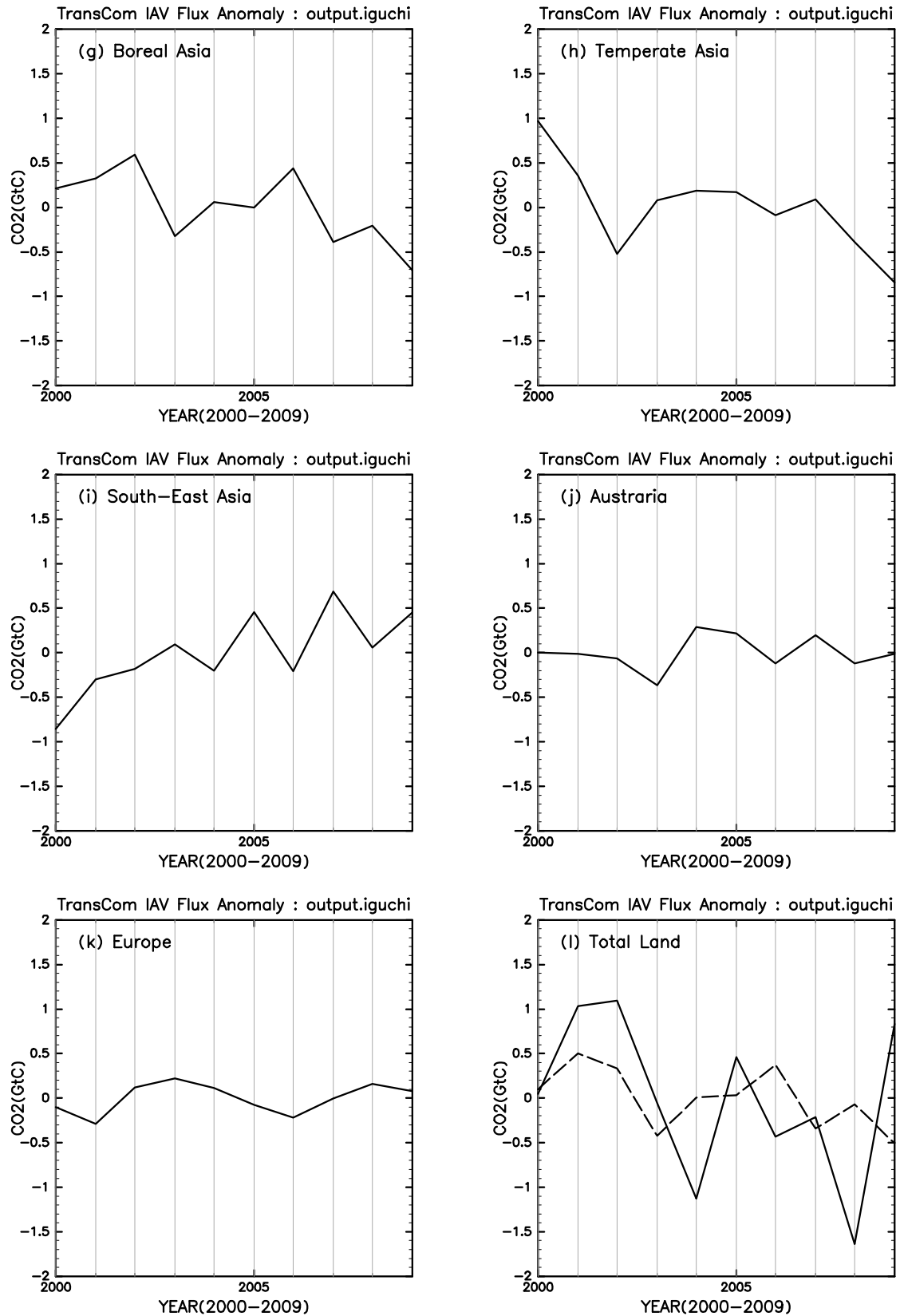
Fig. 2(continued) The dashed line in subfigure (l) is the sum of flux anomalies of (a) and (g).
