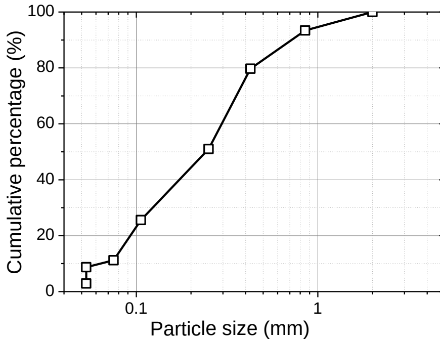
Fig. 3.7 Particle size distributions for C&D waste residue
