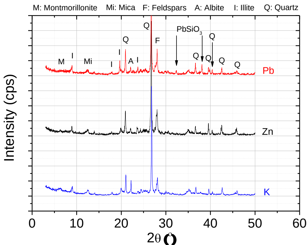
Fig. 4.48 X-ray diffraction patterns of the samples for heavy metals after membrane test
