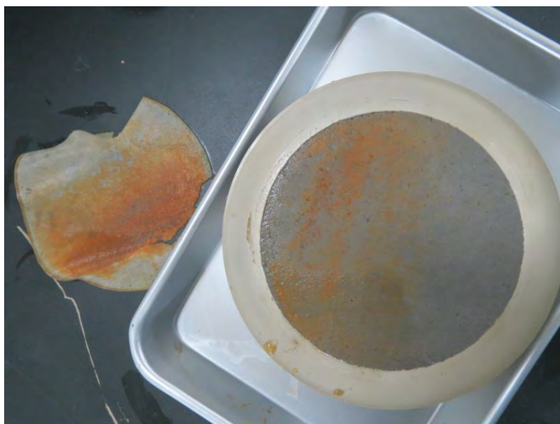
Fig. 4.47 \text{Fe}_2\text{O}_3 at the top side of specimens under alkaline condition after the membrane tests
