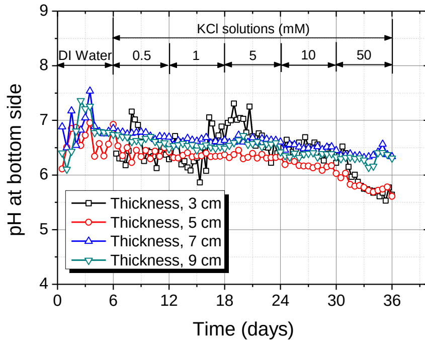
Fig. 4.29 Compare of pH at bottom for specimens with different thickness
