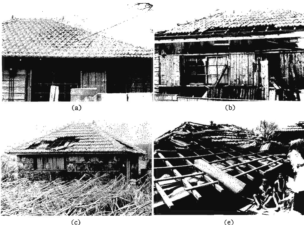
Photo. 5 Damage to wooden building with cement-tile roofing :
