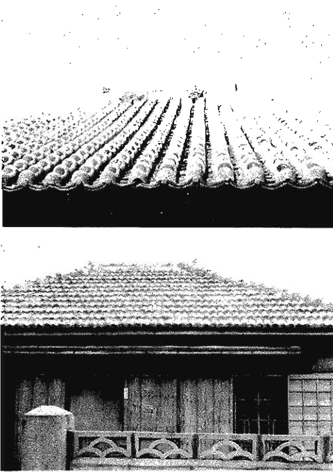
Photo. 1 Two types of roofings of wooden buildings in Okinawa : (a) clay-tile roofing, (b) cement-tile roofing.
