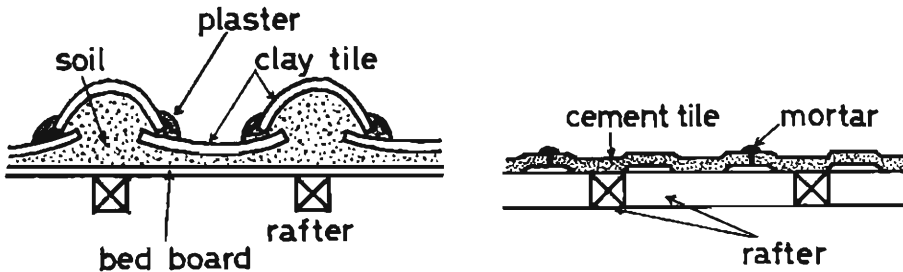
Fig. 1 Two types of roof sections of wooden buildings in Okinawa. (a) clay-tile roofing, (b) cement-tile roofing.
