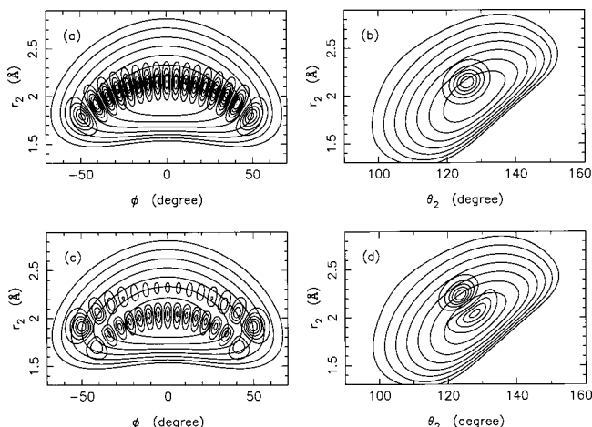
FIG. 5. Plots of the CH chromophore eigenstates: (a) and (b) correspond to the 6_{16} state, while (c) and (d) represent the 1_1 6_{14} state. The contour lines of the potential surface are with the spacing of 10 kcal/mol, from 10 to 70 kcal/mol.
