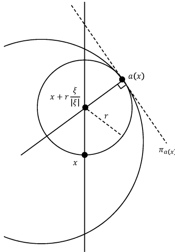
Figure 3. Geometry of the Minkowski functional
