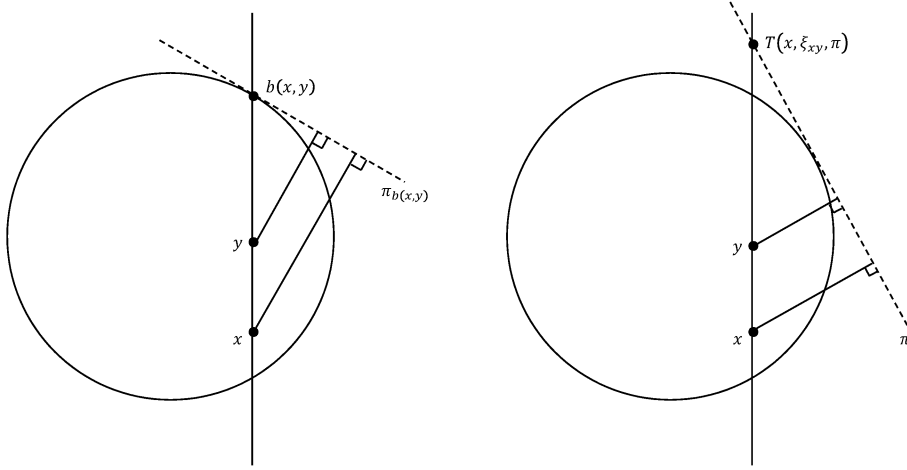
Figure 1. Variations in the pencils of similar triangles
