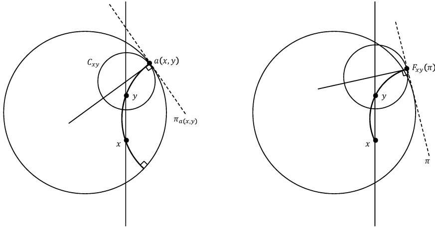
Figure 2. Variations in the pencil of circles
