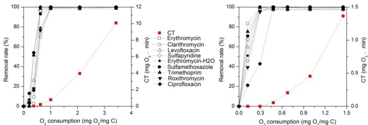
Figure 3.17 Removal of antibiotic compounds during ozonation at different SOC levels (left: SE; right: PE)
