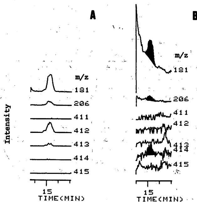
Fig. 4. Mass chromatograms of molecular ion regions and important fragment ions of acetate of methyl oxalate (IX-Ac). A: Unlabeled authentic sample (molecular weight: 412), mass spectral data of which are shown in Table 1-e, B: product of degradation of (II- ^{13}\text{C} ) by Phanerochaete chrysosporium . The chromatograms of m/z 411–415 are magnified five times. Operation conditions of the GC-MS are described in the text.
