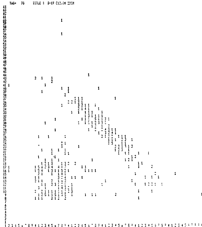
Fig. 1. Two dimensional energy spectrum of the reaction ^{12}\text{C}(^{12}\text{C}, ^8\text{Be})^{16}\text{O} at \theta_L=0^\circ , and E_{\text{lab}}=12.0 MeV.
