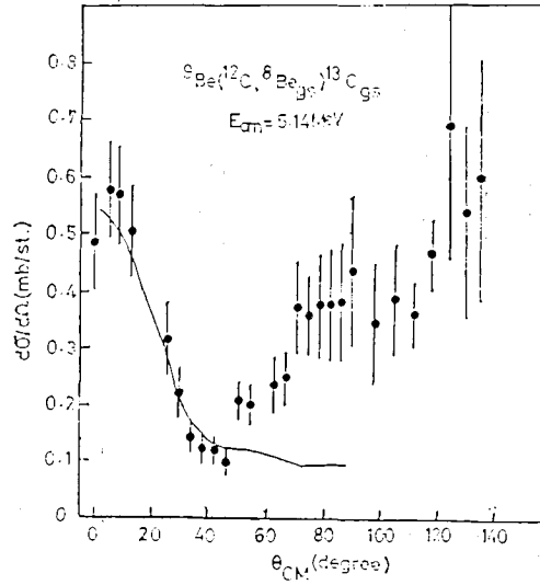
Fig. 10. Resonance analysis of the angular distribution of the {}^9\text{Be}({}^{12}\text{C}, {}^8\text{Be}_{g.s.}){}^{13}\text{C}_{g.s.} reaction at E_{CM}=5.14\text{ MeV} .
