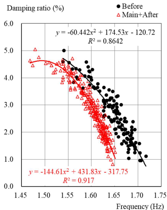
Fig. 41 Correlation between 2nd natural frequency and 2nd modal damping ratio in transverse direction of Building C
