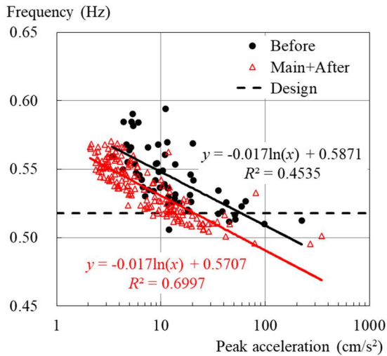
Fig. 2 1st natural frequency depending on peak acceleration on 15th floor in longitudinal direction of Building A
