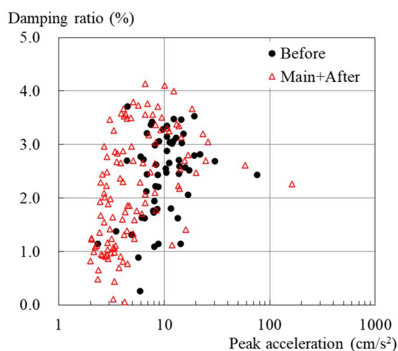
Fig. 28 1st modal damping ratio depending on peak acceleration on 23rd floor in longitudinal direction of Building D
