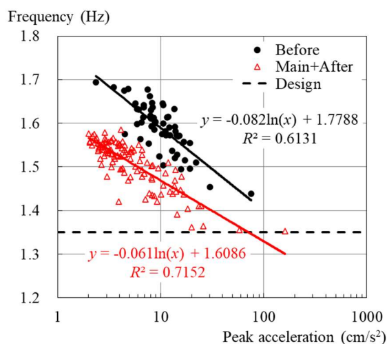
Fig. 27 2nd natural frequency depending on peak acceleration on 23rd floor in longitudinal direction of Building D
