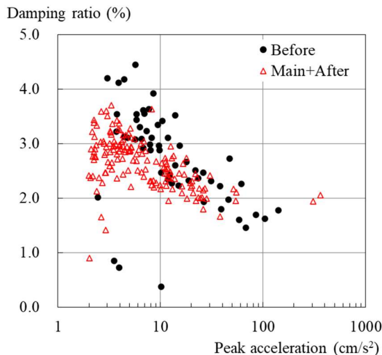
Fig. 8 1st modal damping ratio depending on peak acceleration on 15th floor in transverse direction of Building A
