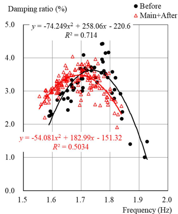
Fig. 33 Correlation between 2nd natural frequency and 2nd modal damping ratio in transverse direction of Building A
