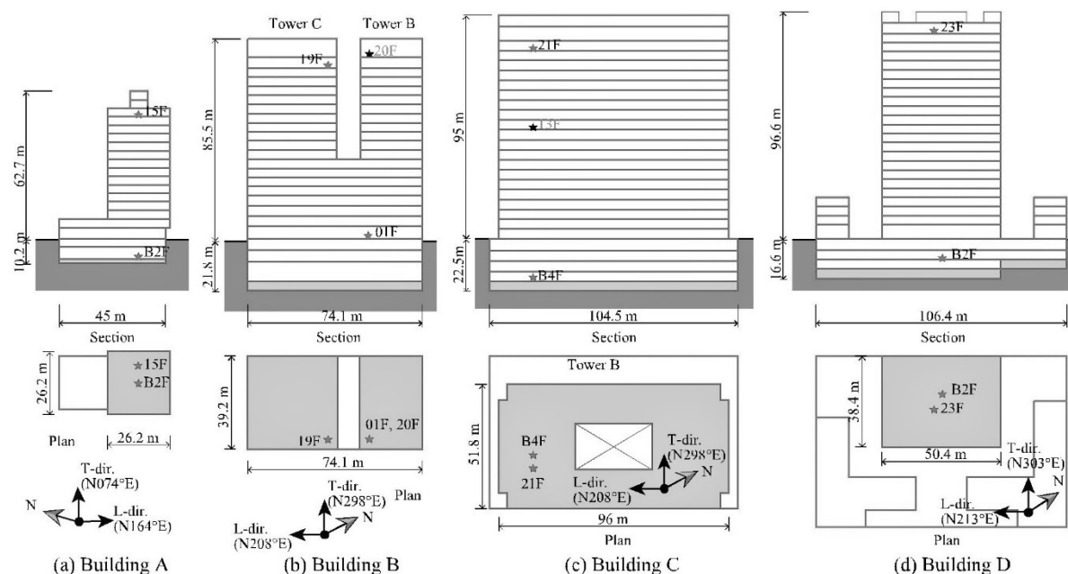
Fig.1 Plans and sectional elevations of buildings
