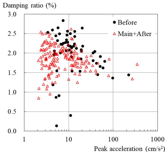
Fig. 4 1st modal damping ratio depending on peak acceleration on 15th floor in longitudinal direction of Building A
