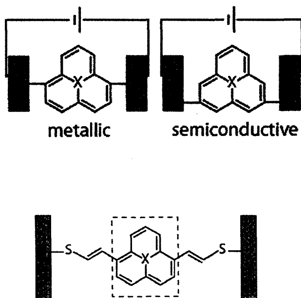
Fig.2 Molecular bridges of Phenalenyl
