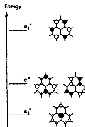
Fig.3 Molecular orbitals of phenalenyl
