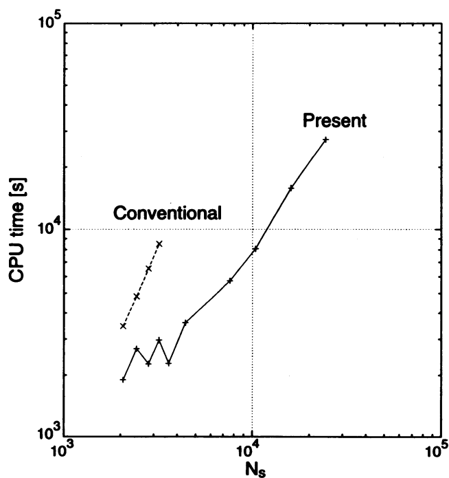
Fig. 5 Comparison of computational time
