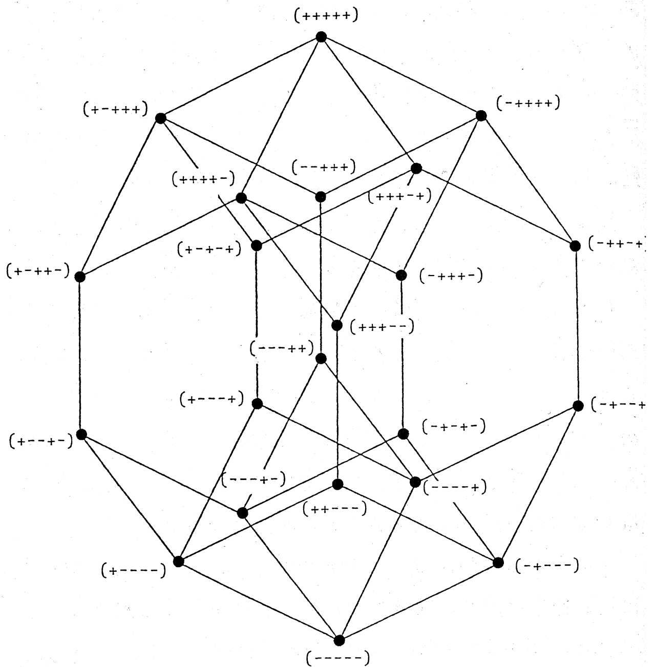
図4. FukudaのAcycloidの極束.
