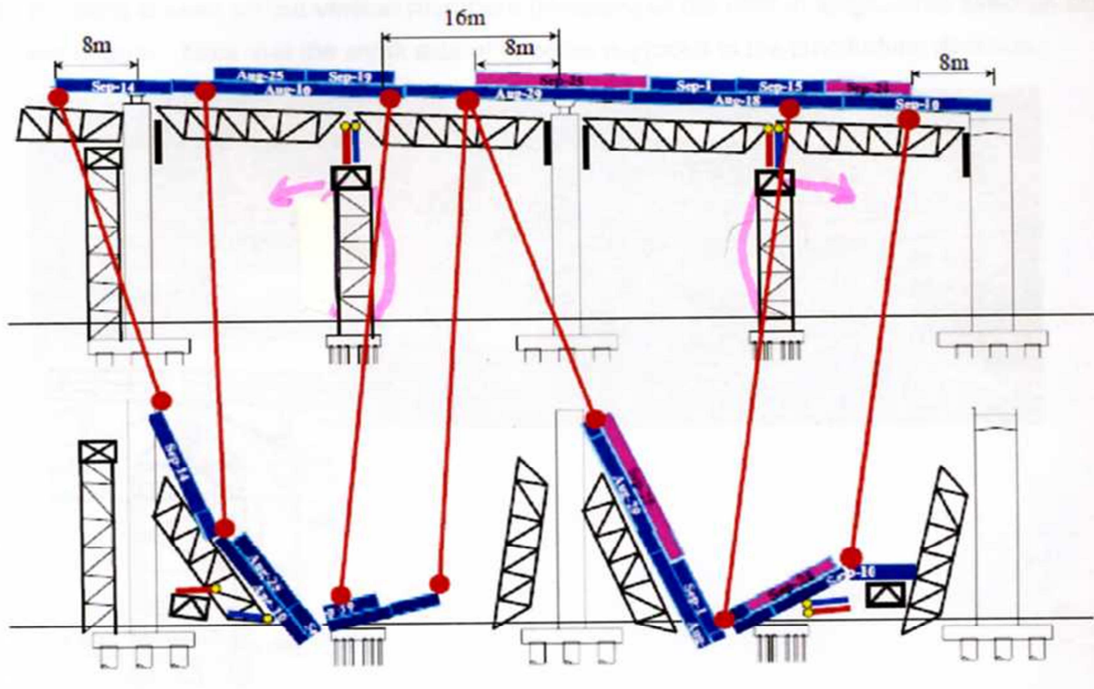
Fig.15 Collapsed concrete segments, scaffoldings and others
