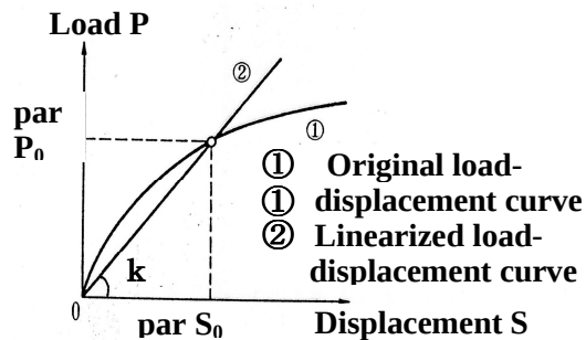
Fig.3 Concept behind the linearization of k
