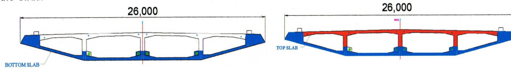
Sections of the Girder
