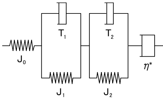
Fig.28 Newly developed model
