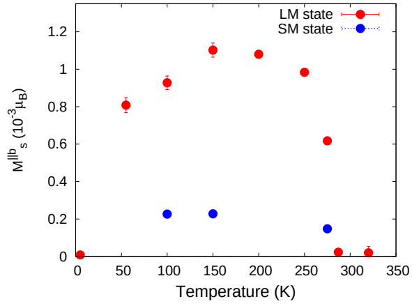
Figure 3.7: Temperature dependences of the spontaneous magnetization along the b-axis M_s^{||b} in the LM and the SM states.
