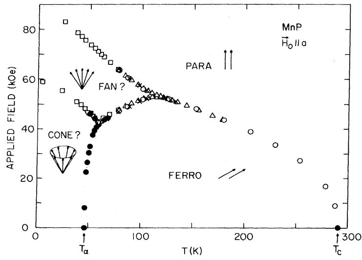
Figure 1.9: H - T magnetic phase diagram in MnP with the magnetic field along the a -axis. "CONE" represents the magnetic phase where the spins incline toward the a -direction with keeping the helical arrangement of their bc -plane component [31].
