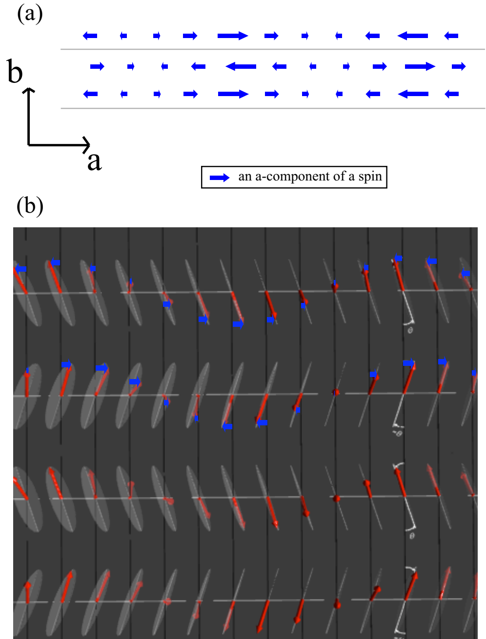
Figure 3.27: (a) The schematic illustration of the (\delta, 1, 0) magnetic modulation. (b) The schematic illustration of the tilted helical structure. The blue arrows in the figures represent the a-components of spins.
