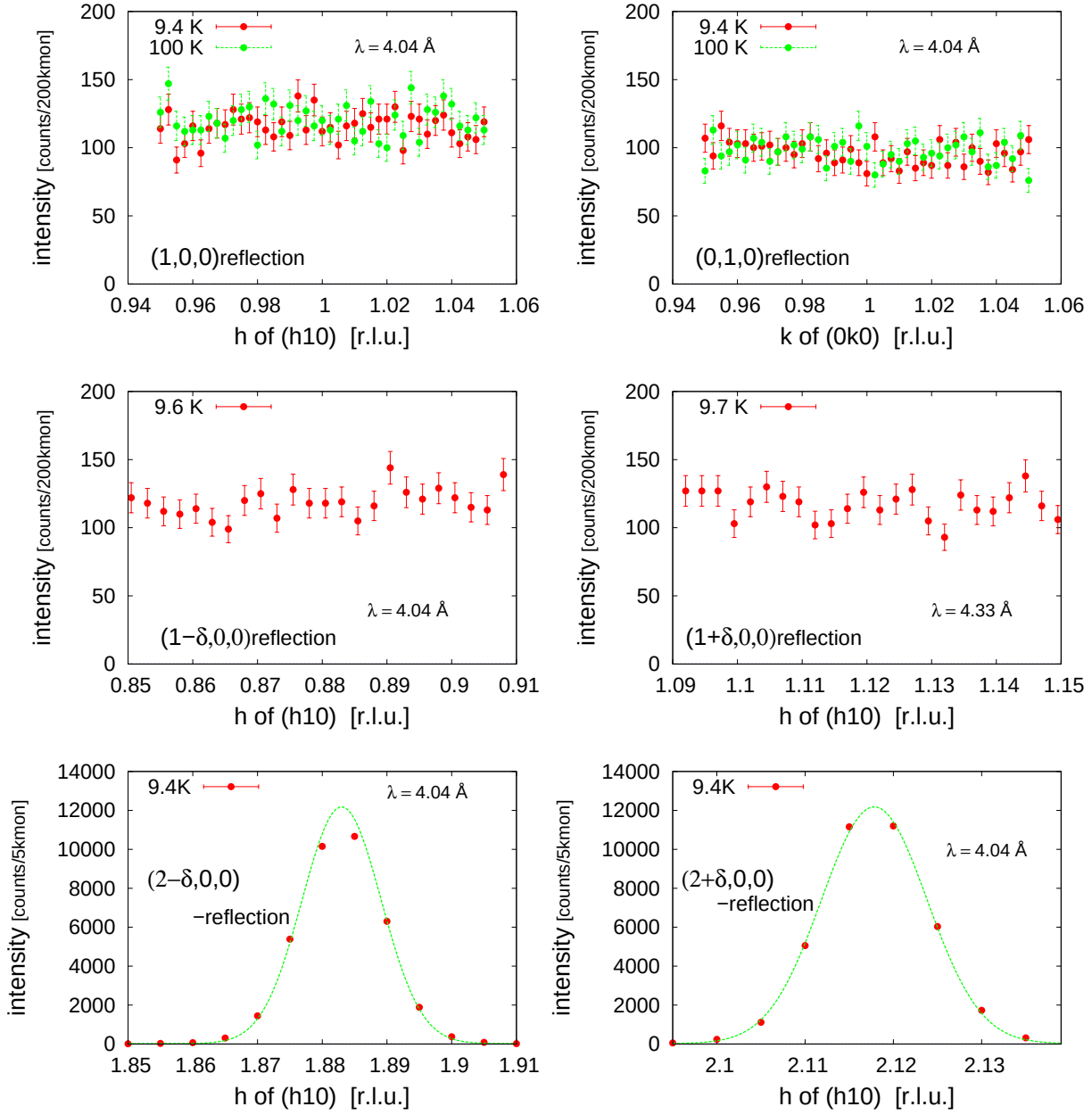
Figure 3.26: The profiles of the (1,0,0), (0,1,0), (1 \pm \delta , 0, 0) and (2 \pm \delta , 0, 0)-reflections.
