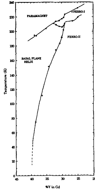
Figure 6.3: Magnetic phase diagram of the \text{Gd}_{1-x}\text{Y}_x alloy series.
