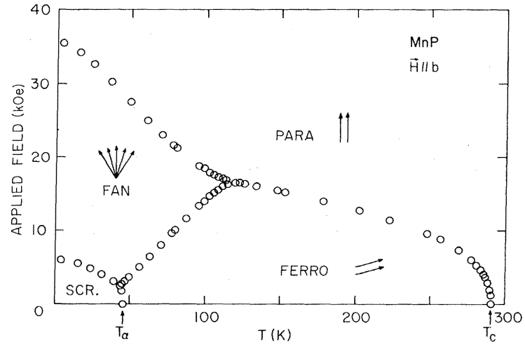
Figure 1.8: H - T magnetic phase diagram in MnP with the magnetic field along the b-axis. "FAN" and "SCR" represent the magnetic phase with the fan-like spin arrangement and the helical phase, respectively [30].
