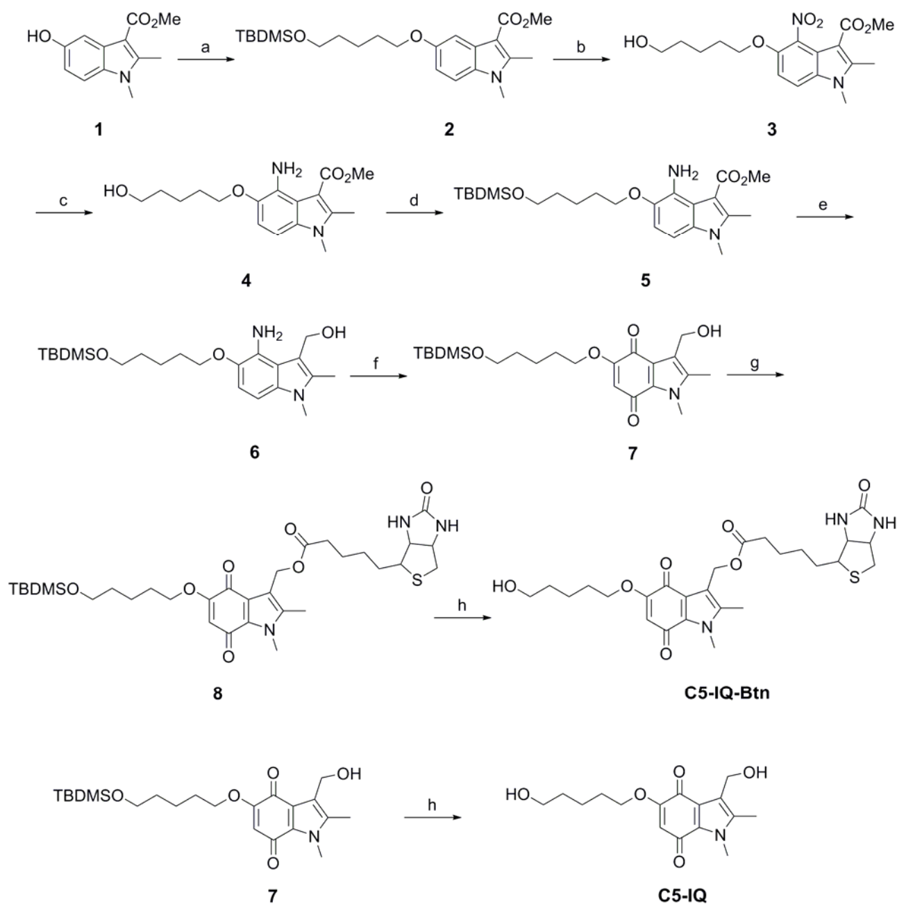
Scheme 1. Reagents and conditions: (a) 5-Bromo-1- tert -butyldimethylsilyloxypentane, NaH, DMF, 0 °C to room temperature, overnight, 38%; (b) HNO 3 , AcOH, CH 2 Cl 2 , 0 °C to room temperature, 4 h, 63%; (c) Sn, HCl, EtOH, reflux at 80 °C, 2 h, 95%; (d) TBDMS-Cl, imidazole, DMF, 0 °C to room temperature, 3.5 h, 85%; (e) LAH, THF, 0 °C, 30 min; (f) Fremy's salt, NaH 2 PO 4 , THF, 0 °C, 20 min, 79% in 2 steps; (g) Biotin, TATU, DIPEA, DMAP, DMF, 0 °C to room temperature, overnight, 93%; (h) AcOH-H 2 O-THF (13:7:3), room temperature, overnight, 81% (C5-IQ-Btn), 90% (C5-IQ).
