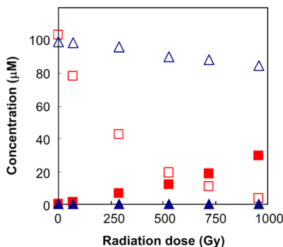
Figure 3. X-Radiolysis (4.0 Gy min -1 ) of IQ-Cou (100 μM; open symbols) in aqueous solution containing 30% 2-methyl-2-propanol at ambient temperature under hypoxic (square) and aerobic (triangle) conditions, with the release of coumarin-3-carboxylic acid (filled symbols).
