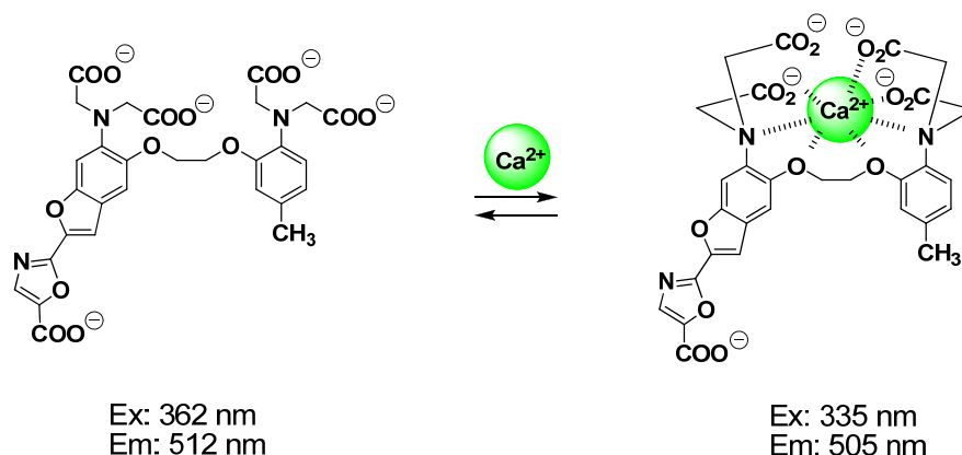
Figure 2. Schematic representation of Fura-2 .
