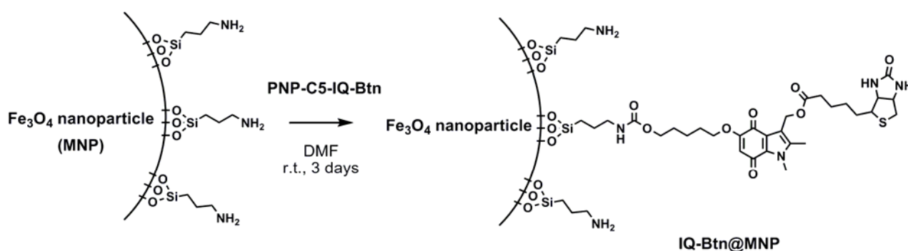
Scheme 1. Synthesis of (A) PNP-C5-IQ-Btn and (B) IQ-Btn@MNP . (A) C5-IQ-Btn , p -nitrophenyl chloroformate (PNP-Cl), triethylamine (TEA), CH 2 Cl 2 , 0 °C to room temperature, 2 h, (33%) (B) PNP-C5-IQ-Btn , DMF, room temperature, 3 days.
