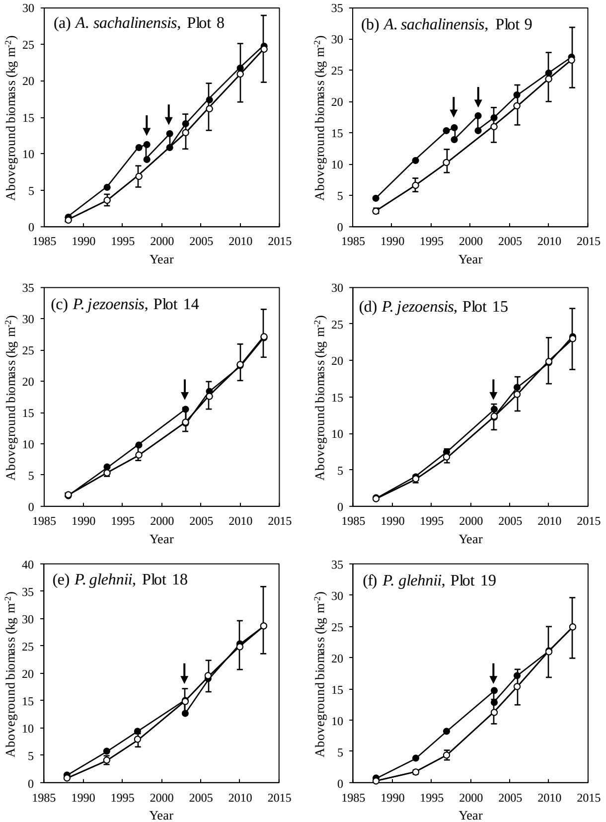
Fig. 3.1 Relationships between reconstructed and observed values of aboveground biomass. ○ and ● represent reconstructed and observed values, respectively. Arrows indicate main years of thinning operations. Solid vertical bars indicate the upper and lower 95% confidence limits of the reconstructed values, based on the bootstrap method
