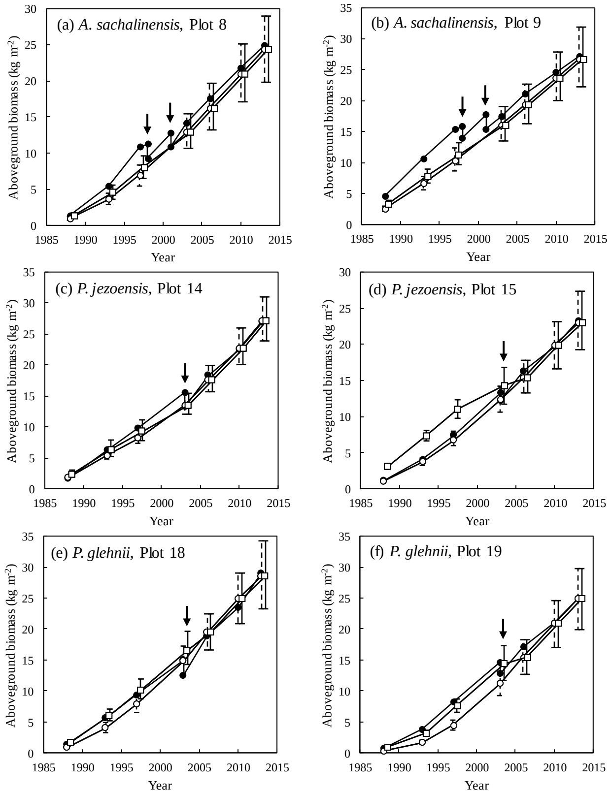
Fig. 4.2 Relationships between reconstructed and observed values of aboveground biomass. \circ , \square , and \bullet , represent reconstructed values using original stand reconstruction, reconstructed values after adding the stumps and observed values, respectively. Arrows indicate main years of thinning operations. Solid and broken vertical bars indicate the upper and lower 95% confidence limits of the reconstructed values with and without stumps, respectively, based on the bootstrap method. The 95% confidence limits cannot be estimated for plot 18 in 1988
