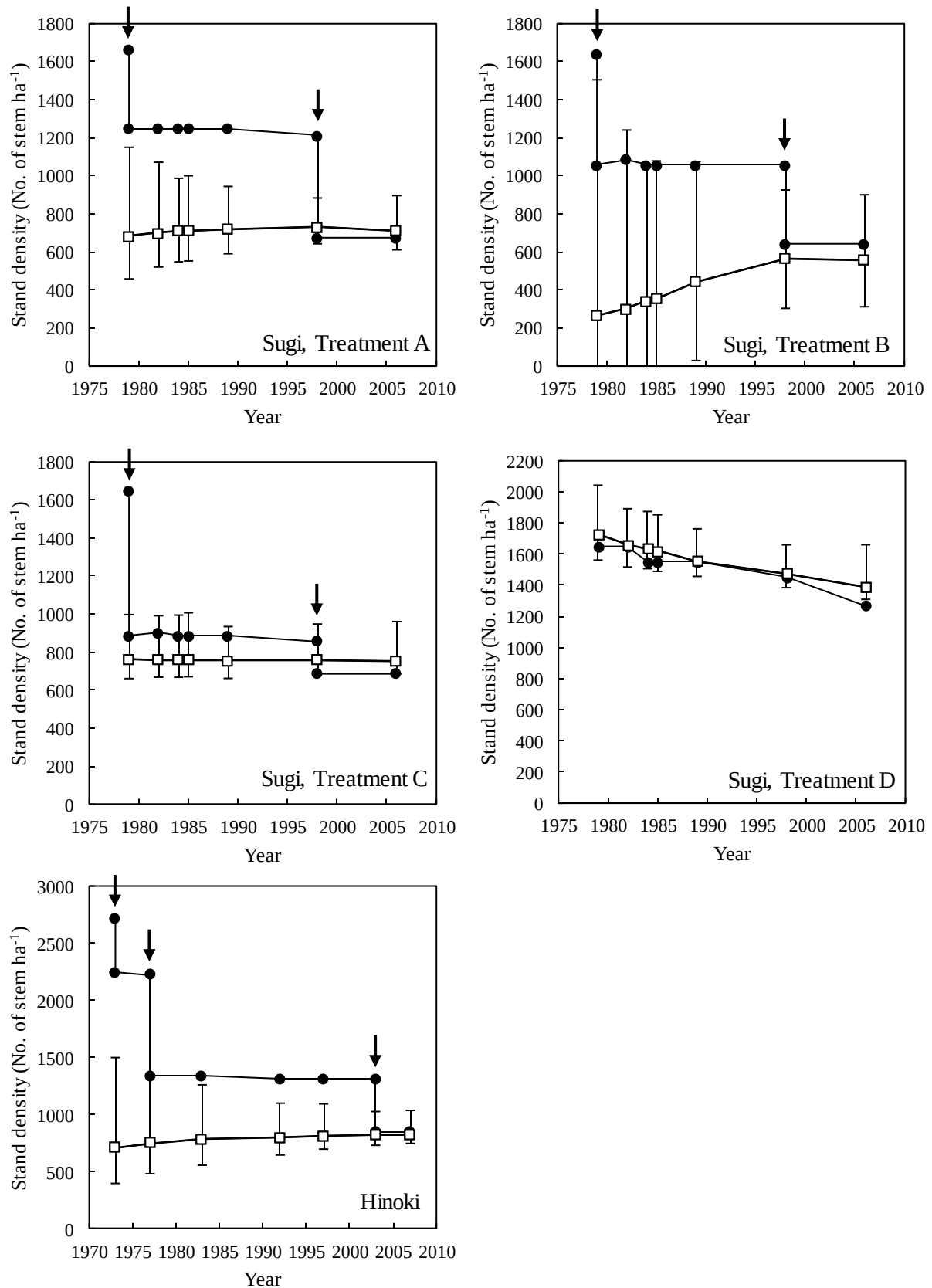
Fig. 2. 4 Relationship between reconstructed and observed values of stand density. □ and ● represent reconstructed values and observed values, respectively. Arrows indicate main years of thinning operations. Solid vertical bars indicate the upper and lower 95% confidence limits of the reconstructed values, based on the bootstrap method
