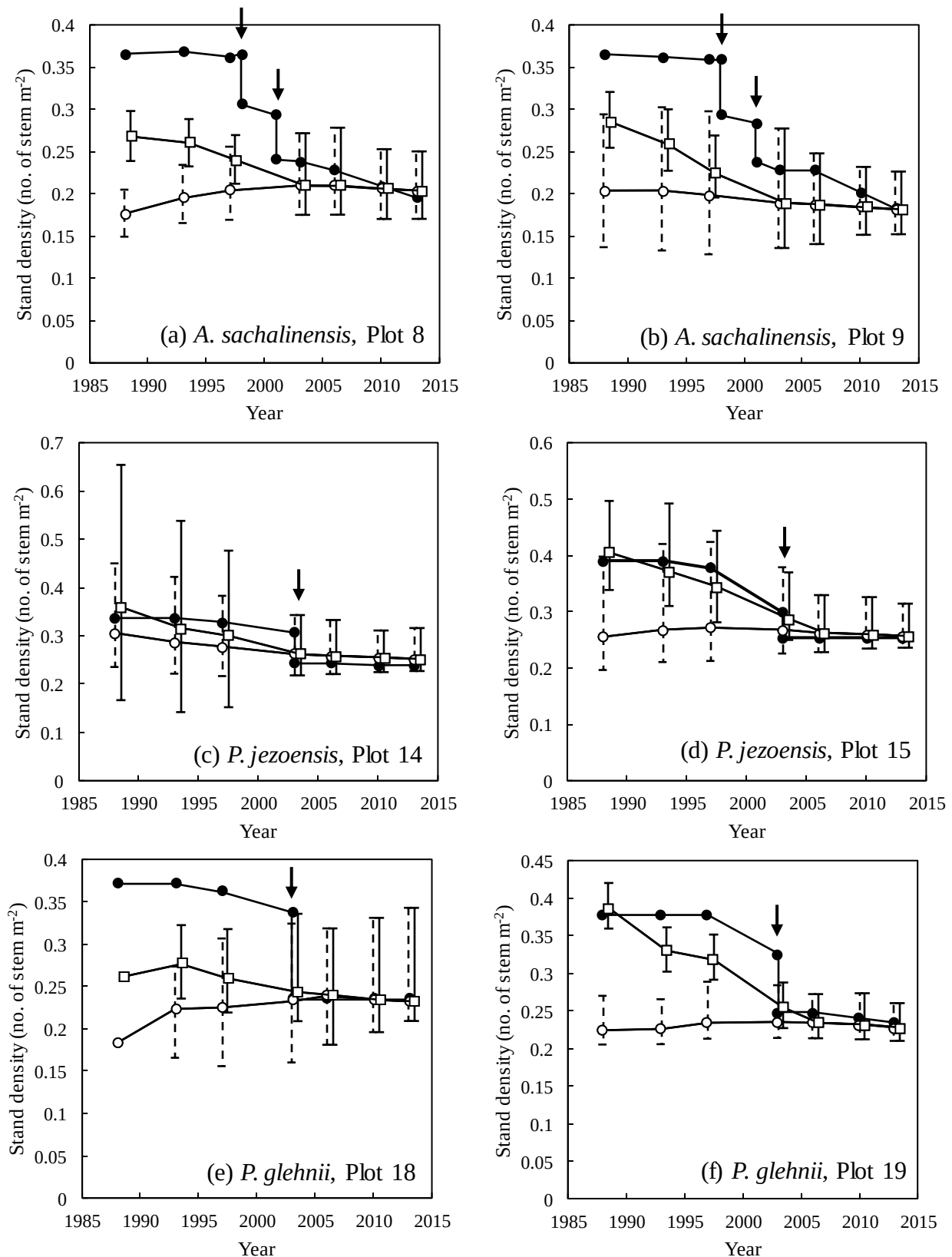
Fig. 4. 5 Relationships between reconstructed and observed values of stand density. ○, □, and ●, represent reconstructed values using original stand reconstruction, reconstructed values after adding the stumps and observed values, respectively. Arrows indicate main years of thinning operations. Solid and broken vertical bars indicate the upper and lower 95% confidence limits of the reconstructed values with and without stumps, respectively, based on the bootstrap method. The 95% confidence limits cannot be estimated for plot 18 in 1988
