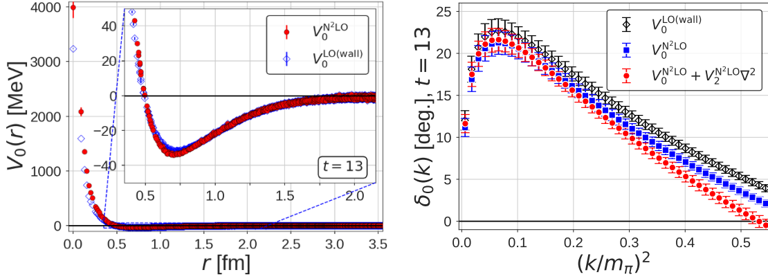
Figure 5. (Left) The LO \Xi\Xi(^1S_0) potential at the N^2 LO analysis, V_0^{N^2LO}(r) (red circles), together with the potential at the LO analysis for the wall source, V_0^{LO(wall)}(r) (blue diamonds) at t/a = 13 on L = 64 . (Right) The scattering phase shifts \delta_0(k) from V_0^{LO(wall)} (black diamonds), V_0^{N^2LO}(r) (blue squares) and V_0^{N^2LO}(r) + V_2^{N^2LO}(r)\nabla^2 (red circles) at t/a = 13 . Both figures from ref. [20].
