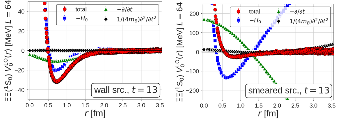
Figure 3. The potential at the leading order (LO) analysis V_0^{\text{LO}}(r) (red circles) from the wall source (left) and the smeared source (right) for \Xi\Xi(^1S_0) at t/a = 13 for L = 64 [20]. The blue squares, green triangles and black diamonds denote 1st, 2nd and 3rd terms in eq. (2.11), respectively.
