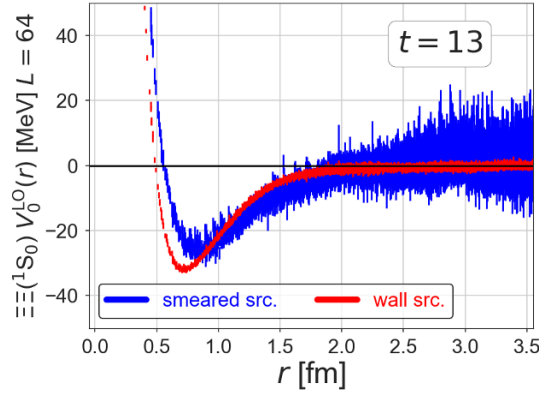
Figure 4. A comparison of the LO \Xi\Xi(^1S_0) potential V_0^{\text{LO}}(r) between the wall source (red) and the smeared source (blue) at t/a = 13 [20].
