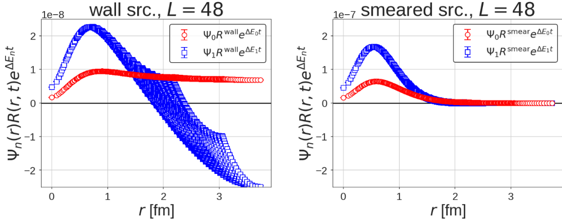
Figure 8. The overlap between the R -correlator and the eigenfunction, \Psi_n^\dagger(\vec{r})R(\vec{r},t)e^{\Delta E_n t} , as a function of r at t/a = 13 on L = 48 for the ground state ( n = 0 , red circles) and the first excited state ( n = 1 , blue squares) in the case of the wall source (left) and the smeared source (right).
