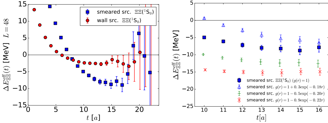
Figure 1. (Left) The source operator dependence of the effective energy shift \Delta E_{\text{eff}}(t) for \Xi\Xi(^1S_0) using the wall source (red circles) and the smeared source (blue squares) for L = 48 [1]. (Right) The sink operator dependence of the same quantity with the smeared source [1].
